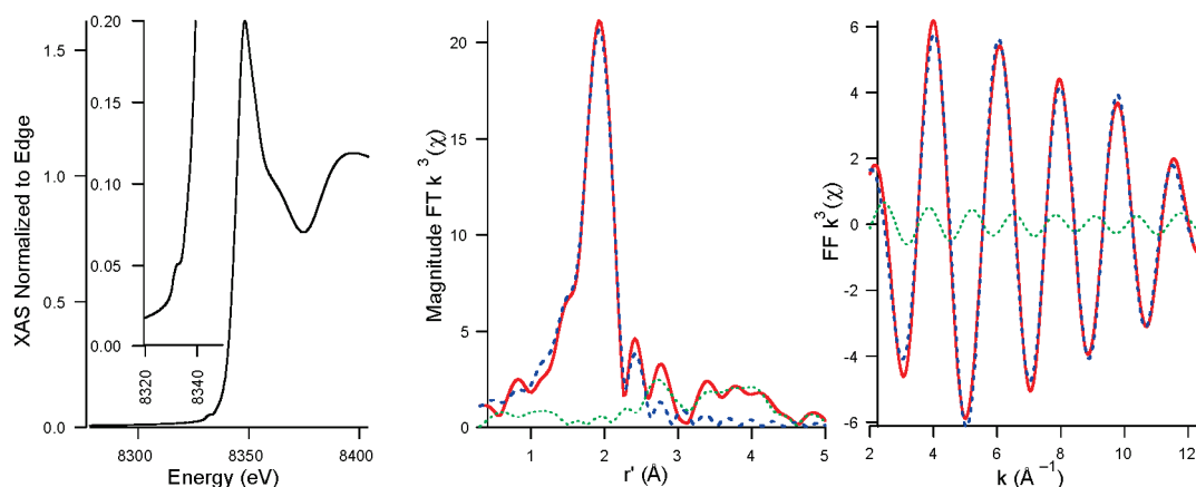
Figure 6. Ni K-edge X-ray absorption data for \text{I}_2 generated \{\text{Ni}^{\text{III}}(\text{SOD}^{\text{M1}}\text{--Im--Me})\} (concentration \sim 3 mM). Experimental data are shown in red, simulations to the data are shown in dashed blue, and the difference spectrum is shown in green. The left figure shows the XANES region of the x-ray absorption (XAS), the middle figure shows the FT k^3 EXAFS, and the right figure shows the FF k^3 EXAFS. The inset presented in the XANES panel displays an expansion of the Ni(1s \rightarrow 3d) transition.
