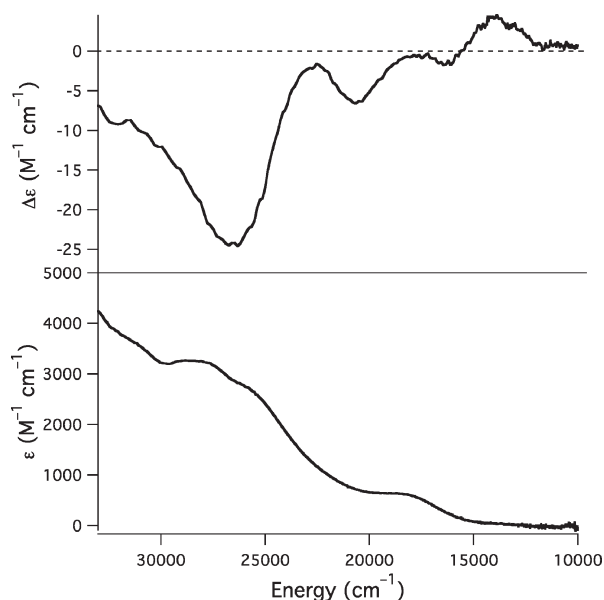
Figure 7. Electronic absorption spectrum (bottom) and CD spectrum (top) of \{\text{Ni}^{\text{III}}(\text{SOD}^{\text{M1}}\text{--Im--Me})\} .
