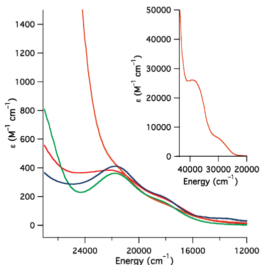
Figure 1. Electronic absorption spectra of \{\text{Ni}^{\text{II}}(\text{SOD}^{\text{M1}}\text{-Im-H})\} (blue trace), \{\text{Ni}^{\text{II}}(\text{SOD}^{\text{M1}}\text{-Im-Me})\} (green trace), \{\text{Ni}^{\text{II}}(\text{SOD}^{\text{M1}}\text{-Im-Tos})\} (red trace), and \{\text{Ni}^{\text{II}}(\text{SOD}^{\text{M1}}\text{-Im-DNP})\} (orange trace). Inset depicts the expanded spectrum of \{\text{Ni}^{\text{II}}(\text{SOD}^{\text{M1}}\text{-Im-DNP})\} .
