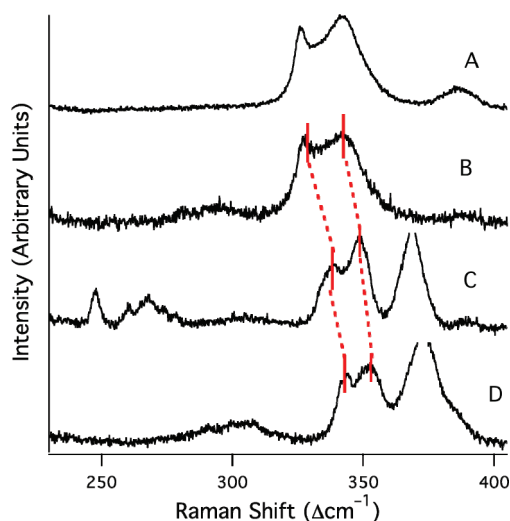
Figure 8. Resonance Raman spectra of \{\text{Ni}^{\text{III}}(\text{SOD}^{\text{M1}}\text{--Im--Me})\} (A and B, recorded at room temperature and 77 K, respectively), \{\text{Ni}^{\text{III}}(\text{SOD}^{\text{M1}}\text{--Im--DNP})\} (C; 77 K), and \{\text{Ni}^{\text{III}}(\text{SOD}^{\text{M1}}\text{--Im--Tos})\} (D; 77 K) following 405 nm excitation. The symmetric N–Ni–S stretching modes are highlighted in red.
