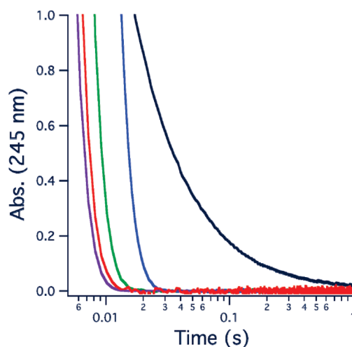
Figure 9. Decay trace for the disproportionation of 50 mM \text{KO}_2 (18-c-6 salt) \{\text{Ni}(\text{SOD}^{\text{M1}}\text{--Im--X})\} (pH 8.0 T = 24.7^\circ\text{C} ). The black trace is the \text{KO}_2 self-disproportionation, the blue trace is \{\text{Ni}(\text{SOD}^{\text{M1}}\text{--Im--Me})\} (60 \mu\text{M} ), the green trace is \{\text{Ni}(\text{SOD}^{\text{M1}}\text{--Im--H})\} (12 \mu\text{M} ), the red trace is \{\text{Ni}(\text{SOD}^{\text{M1}}\text{--Im--DNP})\} (2.0 \mu\text{M} ), and the purple blue trace is \{\text{Ni}(\text{SOD}^{\text{M1}}\text{--Im--Tos})\} (1.0 \mu\text{M} ).
