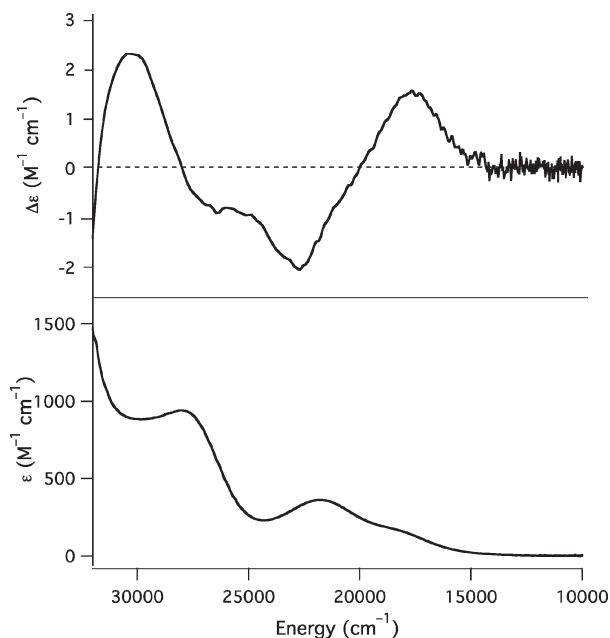
Figure 2. Electronic absorption (bottom) and CD spectrum (top) of \{\text{Ni}^{\text{II}}(\text{SOD}^{\text{M1}}\text{-Im-Me})\} .
