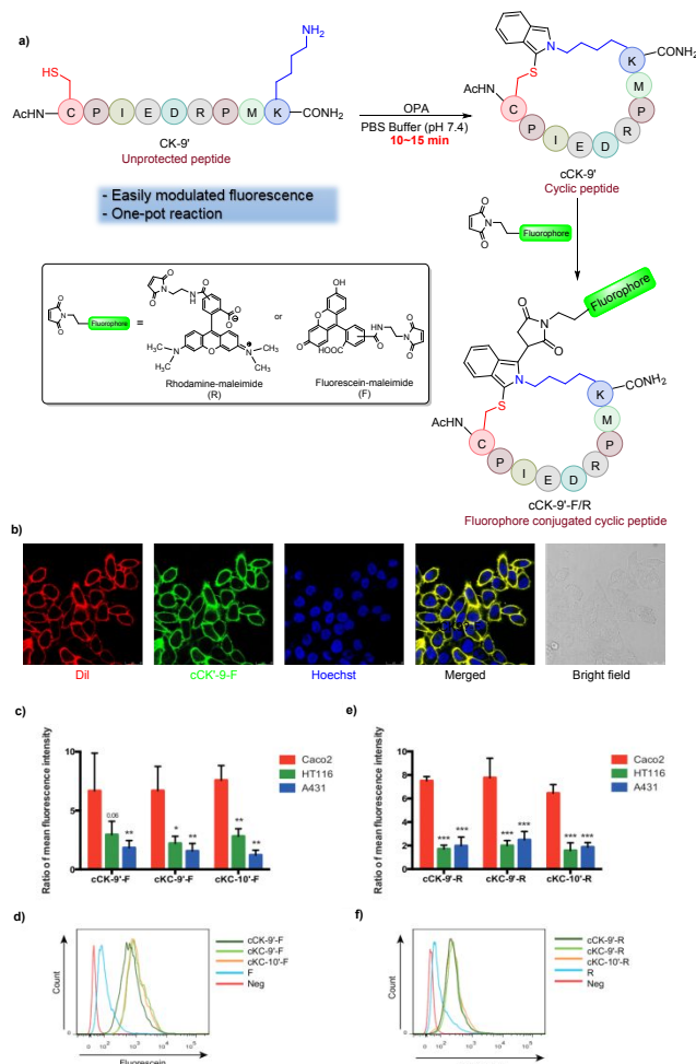
Figure 4. Fluorophore assembled OPA-guided cyclic peptides.
