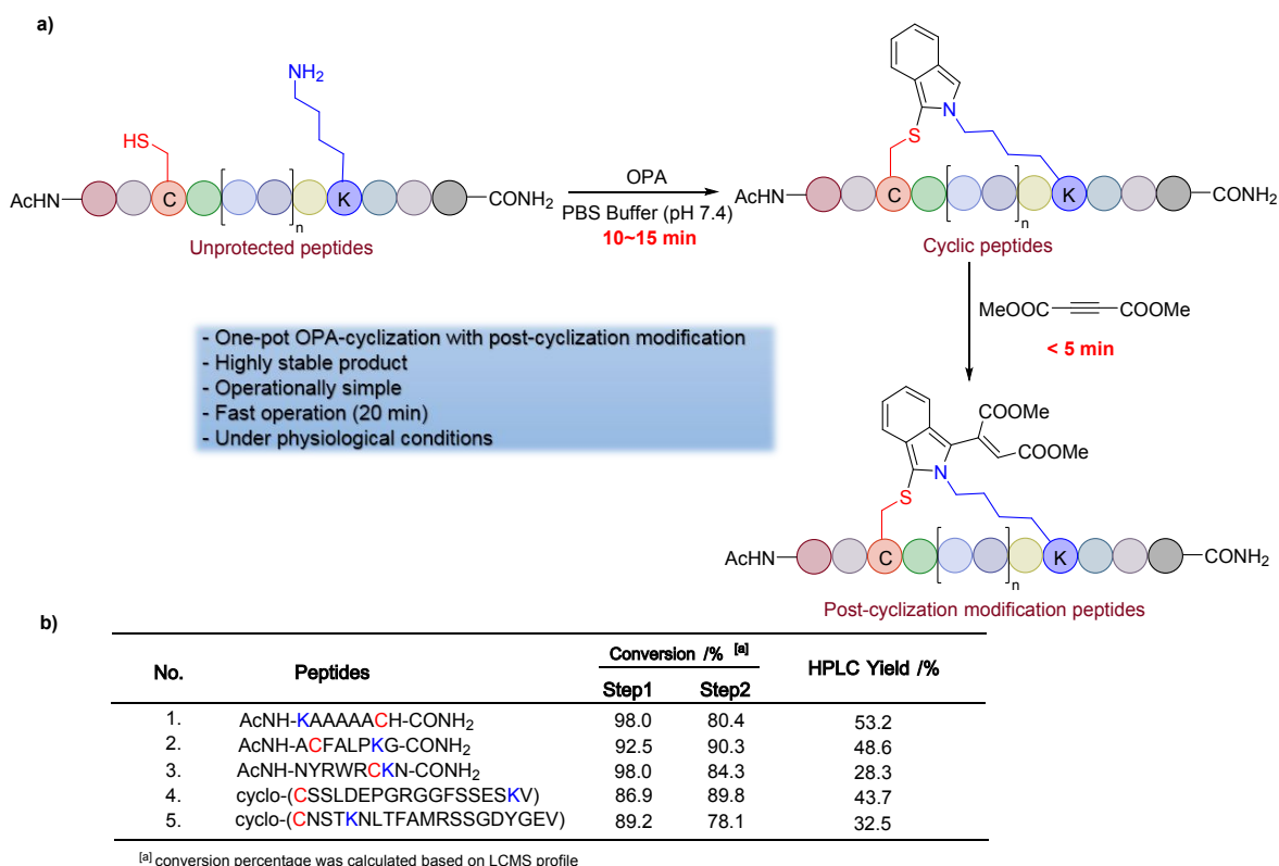
Figure 3. The OPA-guided chemoselective cyclization followed by post-cyclization modification with DMAC. a) Schematic diagram of post-cyclization modification. b) Results of post-cyclization modification with different peptide sequences.
