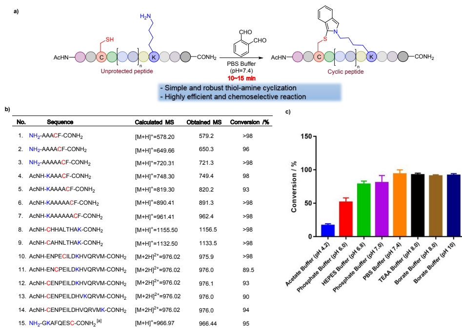
Figure 1. OPA-guided chemoselective cyclization with unprotected peptides. a) Schematic diagram of the OPA-guided chemoselective cyclization. b) The OPA-guided chemoselective cyclization with different peptide sequences. c) The reaction between AcNH-KAAACH-CONH 2 (0.5 mM) and OPA (1 equiv.) under various buffer conditions for 15 min. [a] The ratio of side chain-to-side chain vs. side chain-to-tail cyclization product was roughly 1.7 : 1 based on the NMR and LCMS analysis.
