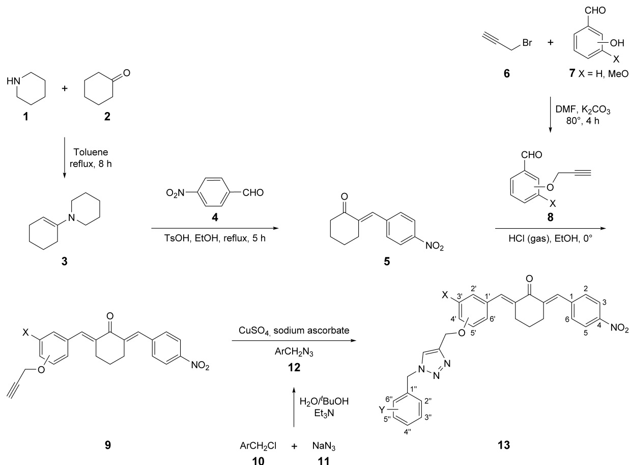
Scheme. Synthesis of novel 1,2,3-triazole-4-linked (2 E ,6 E )-2-benzylidene-6-(4-nitrobenzylidene)cyclohexanones 13
