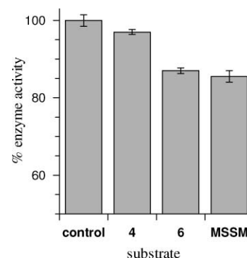
Fig. 2 The effects of myo -inositol on Mtr catalysed substrate turnover: assays were carried out with substrates 4 (400 \mu M), 6 (400 \mu M) and MSSM (105 \mu M) in the presence of myo -inositol (25 mM). Percentage enzyme activities are relative to control experiments (performed separately with each substrate) in the absence of myo -inositol. All assays were carried out in duplicate.
