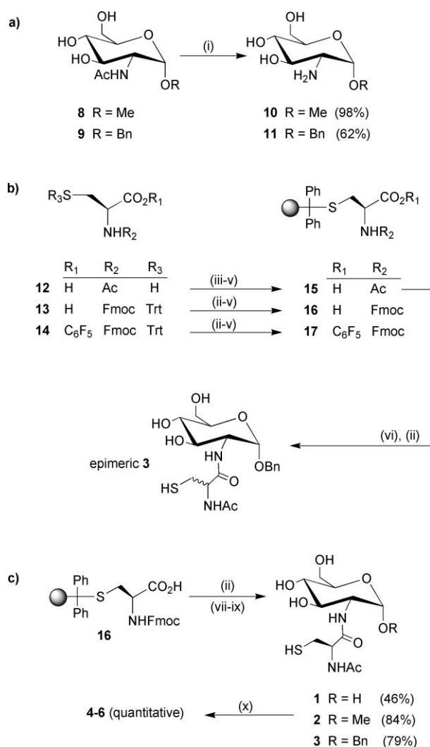
Scheme 1 Reagents and conditions: (i) \text{NH}_2\text{NH}_2 \cdot \text{H}_2\text{O} , 120^\circ\text{C} ; (ii) \text{TFA} - \text{DCM} - \text{Et}_3\text{SiH} (40 : 60 : 3); (iii) polystyrene tritylchloride, DIPEA, \text{CH}_2\text{Cl}_2 - \text{DMF} ; (iv) \text{AcOH} , trifluoroethanol, \text{CH}_2\text{Cl}_2 ; (v) \text{MeOH} , DIPEA, \text{CH}_2\text{Cl}_2 ; (vi) 11 , PyBOP, HOBT, base, \text{DMF} - \text{CH}_2\text{Cl}_2 ; (vii) 10 , 11 or glucosamine (2 eq.), PyBOP, HOBT, 2,6-di- tert -butylpyridine, \text{DMF} - \text{CH}_2\text{Cl}_2 ; (viii) \text{DMF} - \text{piperidine} (8 : 2); (ix) \text{Ac}_2\text{O} (1.1 eq.), pyridine (1.1 eq.), \text{DMF} ; (x) \text{NH}_4\text{HCO}_3 (30 mM), shaking 24–60 h.
