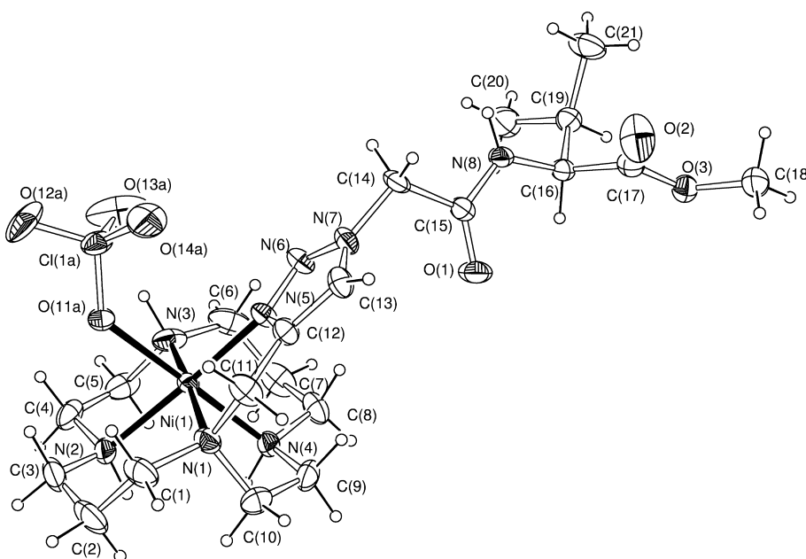
Figure 4. An ORTEP plot of the cation 14ii at the 50% probability level. The noncoordinated perchlorate anion and minor disordered component of the coordinated perchlorate anion are omitted for clarity. Selected bond lengths (Å) and angles (deg): Ni(1)–N(1), 2.159(2); Ni(1)–N(2), 2.101(2); Ni(1)–N(3), 2.079(2); Ni(1)–N(4), 2.0881(19); Ni(1)–N(5), 2.0691(19); Ni(1)–O(11A), 2.2501(16); Ni(1)–O(11B), 2.1150(14); N(1)–Ni(1)–N(2), 91.55(8); N(1)–Ni(1)–N(3), 174.80(8); N(1)–Ni(1)–N(4), 85.39(8); N(1)–Ni(1)–N(5), 81.18(7); N(1)–Ni(1)–O(11A), 89.01(8); N(1)–Ni(1)–O(11B), 101.32(9); N(2)–Ni(1)–N(3), 84.64(9); N(2)–Ni(1)–N(4), 97.19(7); N(2)–Ni(1)–N(5), 170.12(8); N(2)–Ni(1)–O(11A), 83.94(7); N(2)–Ni(1)–O(11B), 88.55(9); N(3)–Ni(1)–N(4), 91.57(8); N(3)–Ni(1)–N(5), 103.02(8); N(3)–Ni(1)–O(11A), 94.10(8); N(3)–Ni(1)–O(11B), 82.16(9); N(4)–Ni(1)–N(5), 88.92(8); N(4)–Ni(1)–O(11A), 174.30(7); N(4)–Ni(1)–O(11B), 171.09(9); N(5)–Ni(1)–O(11A), 89.23(7); N(5)–Ni(1)–O(11B), 86.36(9); O(11A)–Ni(1)–O(11B), 13.25(8). The bond length between metal center and N donor (2.069 Å) is longer than that seen in a comparable complex (2.044 Å) where there is less steric crowding around the metal 43 but shorter than comparable azamacrocyclic complexes based on scorpionand pyridine donors (2.107 Å). 44
