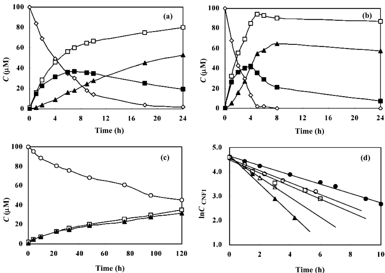
Fig. 2. (a) Concentration vs. time plots for ( \diamond ) CNF1 , ( \square ) 5-FdUrd, ( \blacksquare ) CN3 , and ( \blacktriangle ) CN1 in the hydrolysis of 0.1 mM CNF1 in 10 mM phosphate buffer (PB, pH 7.4) at 37°C. (b) Concentration vs. time plots for ( \diamond ) CNF1 , ( \square ) 5-FdUrd, ( \blacksquare ) CN3 , and ( \blacktriangle ) CN1 in the hydrolysis of 0.1 mM CNF1 in fetal bovine serum (FBS) at 37°C. (c) Concentration vs. time plots for ( \circ ) CNF2 , ( \square ) 5-FdUrd, and ( \blacksquare ) CN2 in the hydrolysis of 0.1 mM CNF2 in 10 mM PB (pH 7.4) at 37°C. (d) First-order kinetic plots for the hydrolysis of CNF1 in ( \bullet ) PB (pH 7.4), ( \circ ) HT-1080 cell lysate, ( \square ) MDA-MB-231 cell lysate, ( \Delta ) FBS, and ( \blacktriangle ) MEM + 10% FBS.
