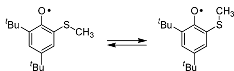
Scheme 5. Possible Conformations for the Radical 1'
