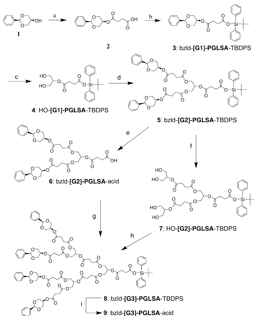
Scheme 1. Synthesis of the [G3]-PGLSA dendron. Reagents and conditions: a) succinic anhydride, pyridine, RT, 18 h, 95 % yield; b) TBDPSi-Cl, imidazole, DMF, RT, 48 h, 86 % yield; c) 20 % Pd(OH) 2 /C, 50 psi. H 2 , THF, RT, 3 h, 95 % yield; d) 2, DCC, DPTS, DCM, RT, 18 h, 88 % yield; e) TBAF, THF, 1 h, RT, 87 % yield; f) 20 % Pd(OH) 2 /C, 50 psi. H 2 , THF, RT, 3 h, 95 % yield; g) 4, DCC, DPTS, DCM, RT, 18 h, 83 % yield; h) 2, DCC, DPTS, DCM, RT, 18 h, 54 % yield; i) TBAF, THF, 1 h, RT, 83 % yield.
