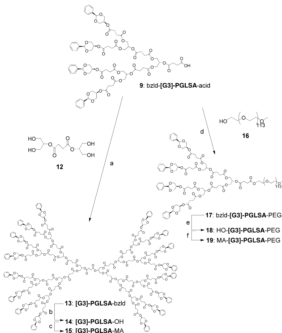
Scheme 3. Synthesis of the [G3]-PGLSA dendrimer and dendritic-linear hybrid. Reagents and conditions. a) DCC, DPTS, DCM, RT, 72 h, 73 % yield; b) 20 % Pd(OH) 2 /C, 50 psi. H 2 , THF, RT, 3 h, 97 % yield; c) methacrylic anhydride, DMAP, DCM, 4.5 h, RT, 64 % yield; d) DCC, DPTS, DCM, RT, 168 h, 89 % yield; e) 20 % Pd(OH) 2 /C, 50 psi. H 2 , THF, RT, 3 h, 83 % yield; f) methacrylic anhydride, DMAP, DCM, RT, 18 h, 96 % yield. MA = methacrylate.
