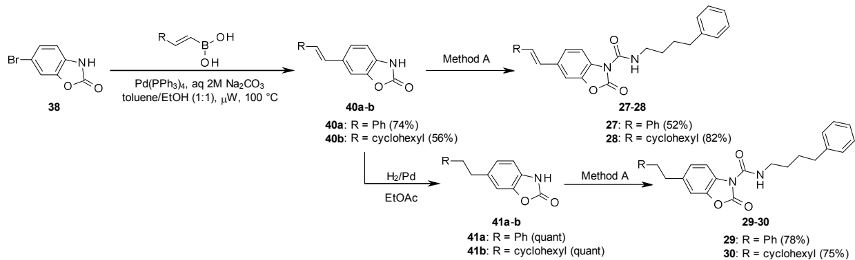
Scheme 3. Synthesis of 6-substituted benzoxazolone carboxamides 27-30
