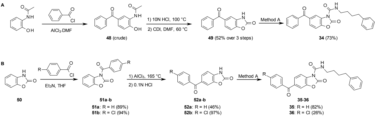
Scheme 5. Synthesis of benzoyl-benzoxazolone carboxamides 34-36
