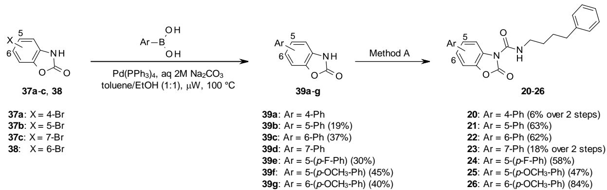
Scheme 2. Synthesis of phenyl-substituted benzoxazolone carboxamides 20-26
