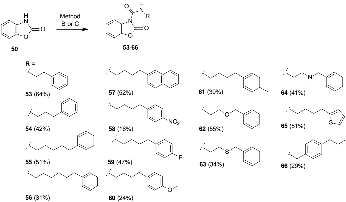
Scheme 6. Synthesis of benzoxazolone carboxamide derivatives 53-66
