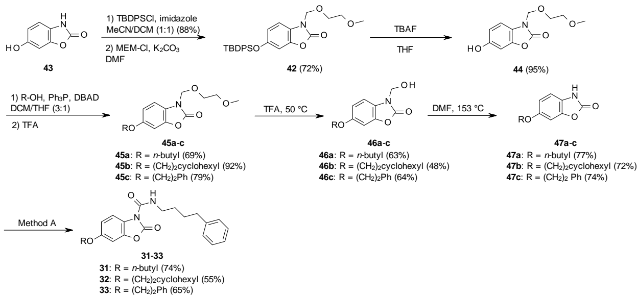
Scheme 4. Synthesis of 6-alkoxy benzoxazolone carboxamides 31-33
