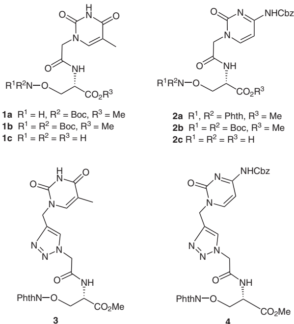
Figure 1 Structures of the target nucleo aminooxy acid derivatives
