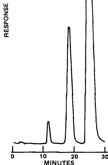
Figure 1—High-pressure liquid chromatogram of the equilibrium mixture of I. The pH of the mobile phase was 2.5.
