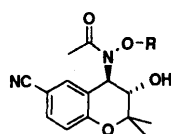
Va, Y-27152 (R = Bn) Vb, Y-26763 (R = H)
