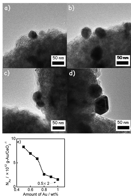
Figure 2. TEM images of MS-Au(X)/CeO 2 samples with various Au contents (X): (a) 0.5 wt %, (b) 0.7 wt % (= 0.5 + 0.1 × 2), (c) 0.8 wt % (= 0.5 + 0.1 × 3), and (d) 1.0 wt % (= 0.5 + 0.1 × 5). (e) Effect of X on N Au .
