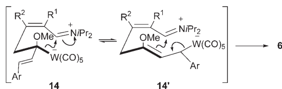
Scheme 6. Mechanistic proposal for the formation of cyclopentenamine derivatives 6 .
