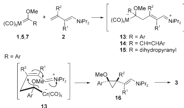
Scheme 5. Mechanistic proposal for the formation of cyclopropane derivatives 3 .
