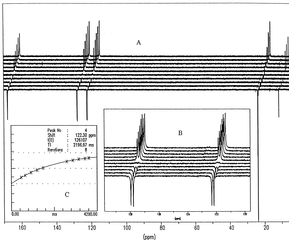
Fig. 2. A = full scale ^{31}\text{P}\{^1\text{H}\} stacked inversion recovery experiment; B = expansion of P(III) resonance region (see Section 4 for details of acquisition parameters); C = exponential plot of signal intensity versus delay time for the resonance at \delta_p 122.3 ppm.
