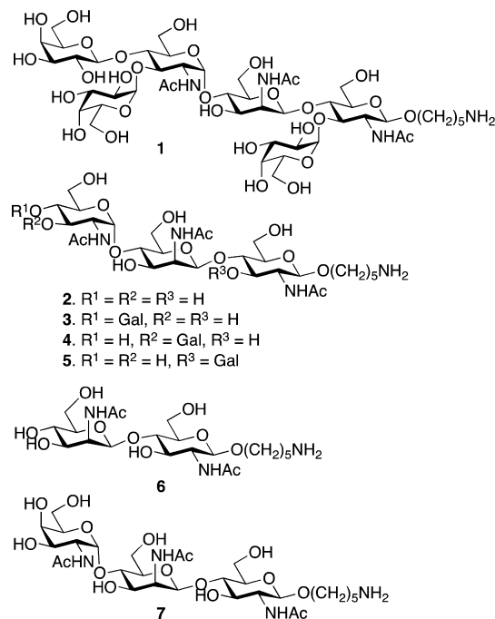
Figure 2. Synthetic targets for binding studies.
