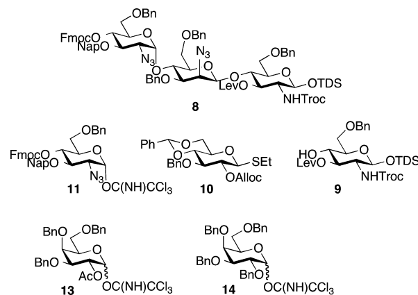
Figure 3. Building blocks for assembly of oligosaccharides.
