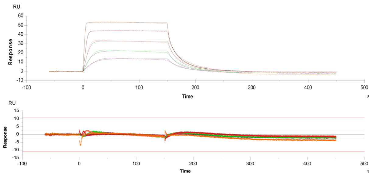
Figure 4. Sensorgram representing the concentration-dependent kinetic analysis of the binding of trisaccharide 2 with immobilized PlyL. It shows the simultaneous kinetic analysis of 2-fold serial dilutions of 2 at concentrations of 100 to 6.25 \mu\text{M} , fitted with a Langmuir 1:1 binding model (black lines).
