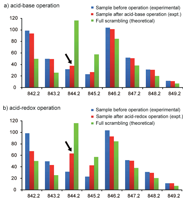
Figure 6. Results of the crossover study on the processivity of the C_5 system: (a) acid–base operation over two cycles; (b) acid–redox operation over two cycles (see Scheme 4). Shown are the (normalized) isotopic distributions of the 1:1 mixture before operation (blue; experimental), after operation (red; experimental), and the distribution that would be expected when full statistical scrambling occurred (green; theoretical). The distribution (red bars and blue bars) of experimental data points is the average of 10 runs for each experiment. This procedure demonstrated the reproducibility of the mass spectrometry data and enabled the isotope scrambling to be analyzed for statistical significance (see the Supporting Information).
