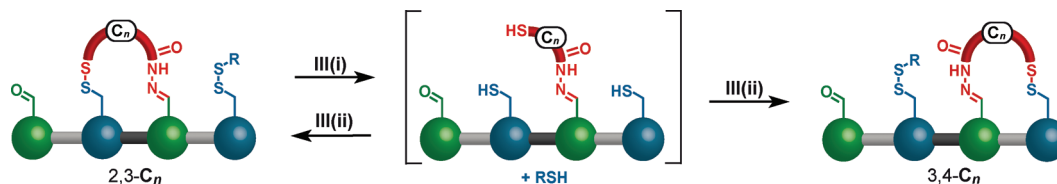
Scheme 3. Kinetically Controlled Redox Operation for Disulfide Exchange, Illustrated for 2,3- C_n a
