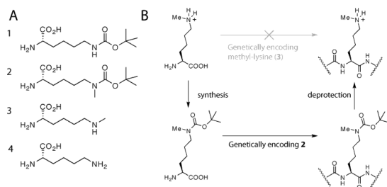
Figure 1. Strategies for encoding lysine methylation. (A) Amino acids used. (B) Schemes for encoding 3 in recombinant proteins.
