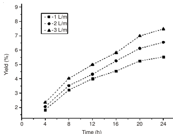
Fig. 6. Yield of diphenyl methanone from oxidation of the diphenylmethane under different airflow at 353 K
