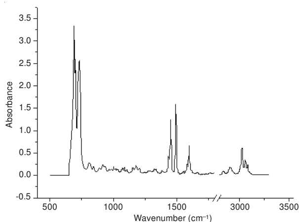
(a) Diphenyl methane
