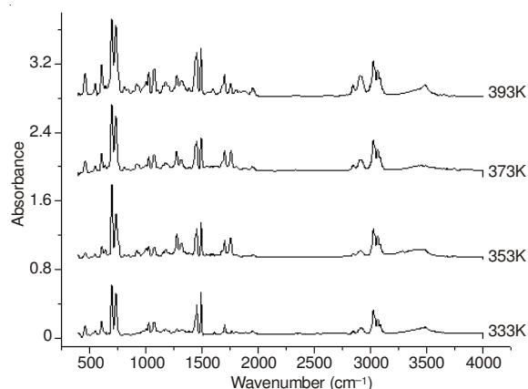
(b) Diphenyl methane after oxidized 24 h
