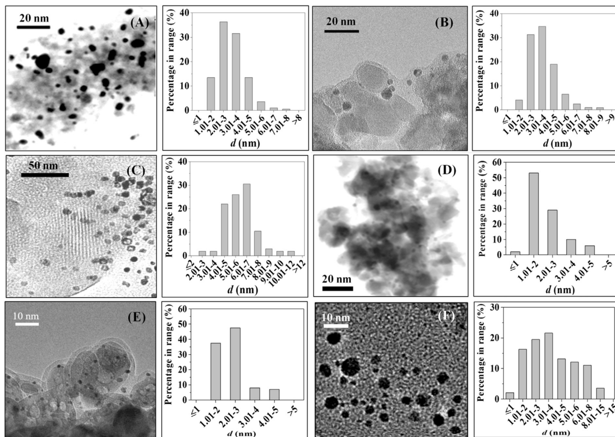
Fig. 4. Representative TEM/STEM images of (A) Au/ \gamma -Al 2 O 3 , (B) Au/TiO 2 , (C) Au/ZrO 2 , (D) Au/CeO 2 , (E) Au/ \alpha -Fe 2 O 3 and (F) Au/Fe 3 O 4 with associated Au size distribution histograms.
