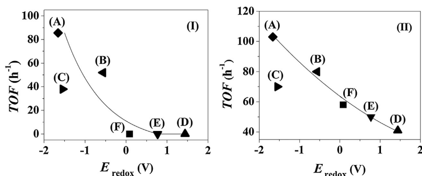
Fig. 8. Dependence of turnover frequency (TOF) on the standard redox potential of the oxide supports ( E_{\text{redox}} from [38]) in (I) benzaldehyde and (II) nitrobenzene hydrogenation: (A) \blacklozenge Au/ \gamma - \text{Al}_2\text{O}_3 ; (B) \blacktriangleleft Au/TiO 2 ; (C) \blacktriangleright Au/ZrO 2 ; (D) \blacktriangle Au/CeO 2 ; (E) \blacktriangledown Au/ \alpha -Fe 2 O 3 ; (F) \blacksquare Au/Fe 3 O 4 .
