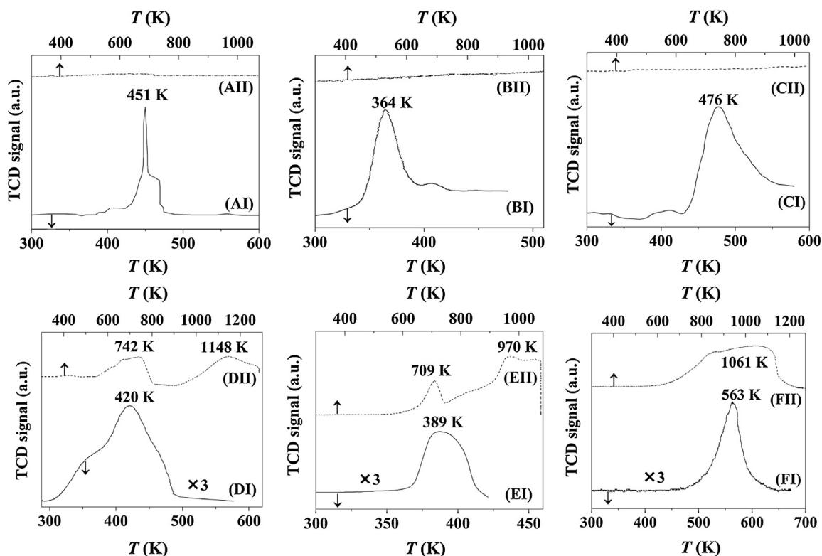
Fig. 1. Temperature programmed reduction (TPR) profiles for (I) supported Au (solid lines) and (II) the corresponding supports (dotted lines): (A) \gamma - \text{Al}_2\text{O}_3 , (B) \text{TiO}_2 , (C) \text{ZrO}_2 , (D) \text{CeO}_2 , (E) \alpha - \text{Fe}_2\text{O}_3 , (F) \text{Fe}_3\text{O}_4 .
