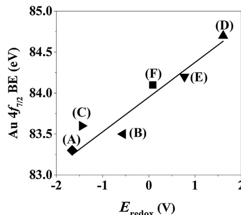
Fig. 6. Dependence of Au 4f 7/2 binding energy (BE) on the standard redox potential ( E_{\text{redox}} ) of the oxide supports: (A) \blacklozenge Au/γ-Al 2 O 3 ; (B) \blacktriangleleft Au/TiO 2 ; (C) \blacktriangleright Au/ZrO 2 ; (D) \blacktriangle Au/CeO 2 ; (E) \blacktriangledown Au/α-Fe 2 O 3 ; (F) \blacksquare Au/Fe 3 O 4 .
