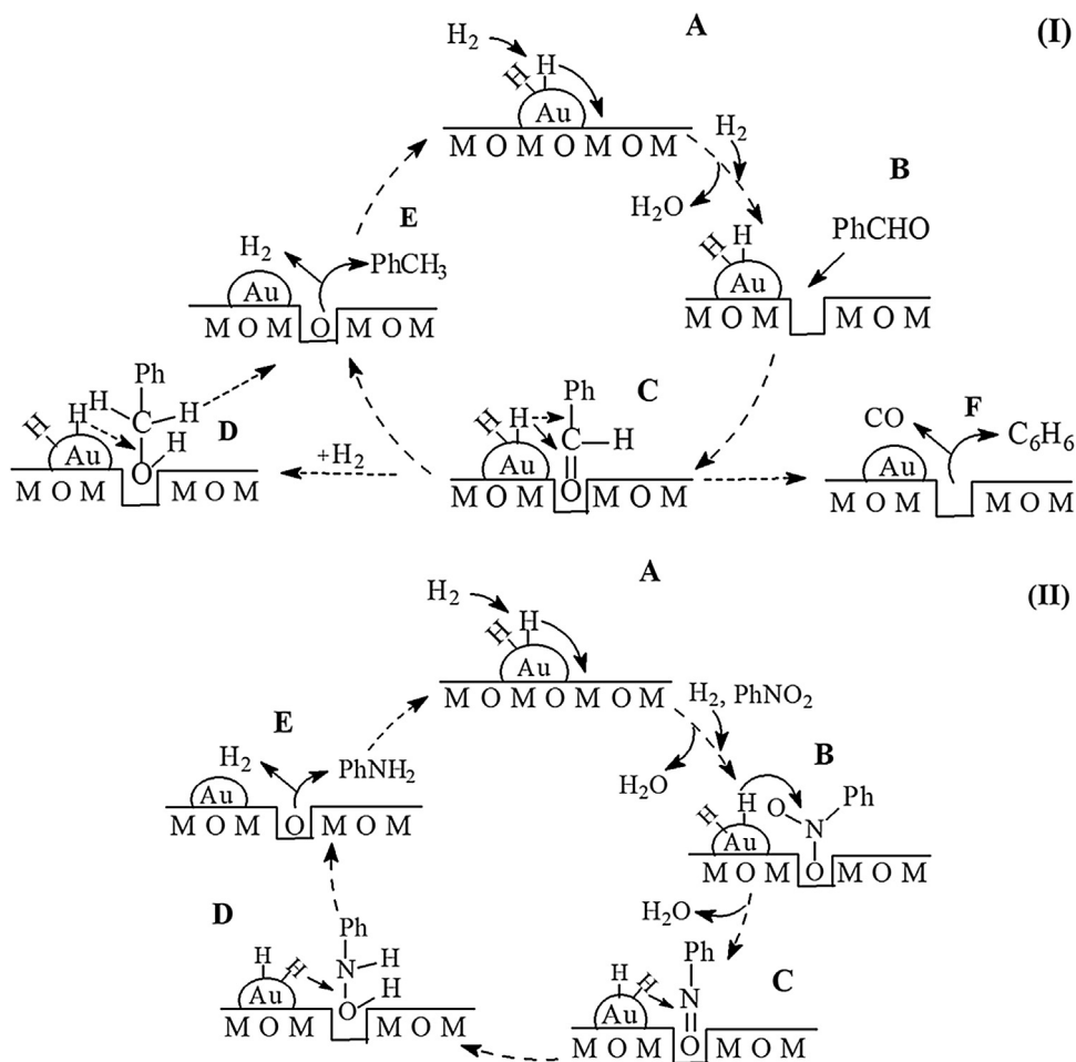
Fig. 9. Proposed reaction mechanism for (I) benzaldehyde and (II) nitrobenzene hydrogenation over Au on reducible supports; M = Ce or Fe.
