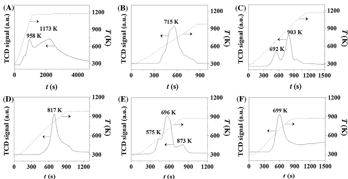
Fig. 2. Hydrogen temperature programmed desorption (TPD) profiles: (A) Au/ \gamma - \text{Al}_2\text{O}_3 , (B) Au/ \text{TiO}_2 , (C) Au/ \text{ZrO}_2 , (D) Au/ \text{CeO}_2 , (E) Au/ \alpha - \text{Fe}_2\text{O}_3 , (F) Au/ \text{Fe}_3\text{O}_4 .
