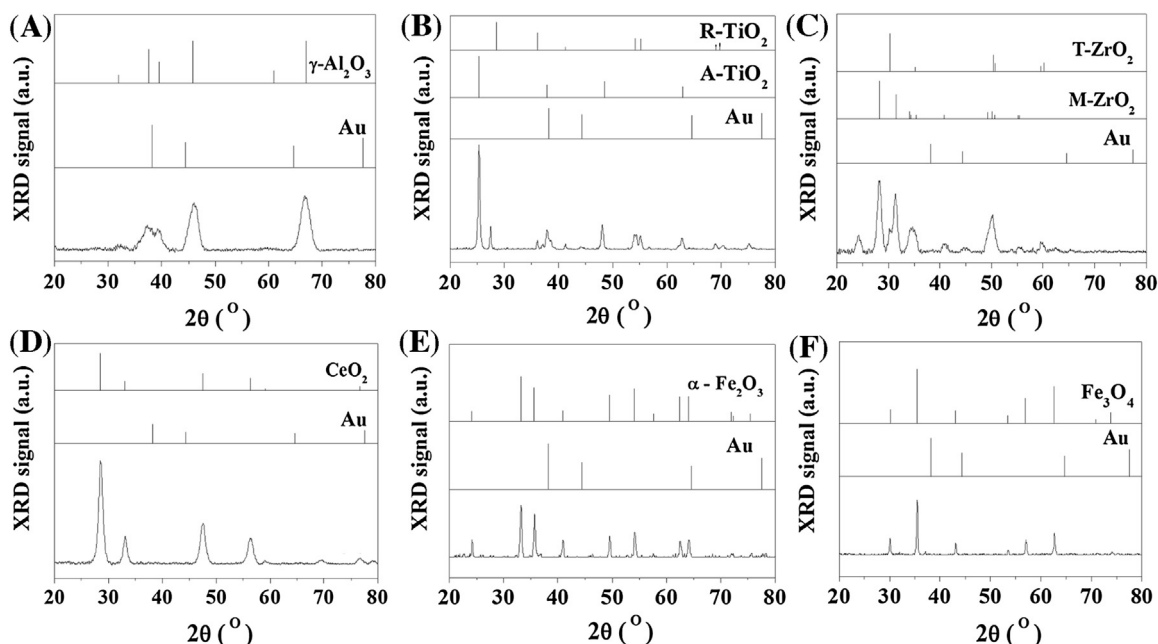
Fig. 3. XRD patterns for activated/passivated (A) Au/ \gamma -Al 2 O 3 , (B) Au/TiO 2 , (C) Au/ZrO 2 , (D) Au/CeO 2 , (E) Au/ \alpha -Fe 2 O 3 and (F) Au/Fe 3 O 4 ; reference JCPDS-ICDD patterns (see card No. in Section 2.2) are included for Au, \gamma -Al 2 O 3 , anatase TiO 2 (A-TiO 2 ), rutile TiO 2 (R-TiO 2 ), monoclinic ZrO 2 (M-ZrO 2 ), tetragonal ZrO 2 (T-ZrO 2 ), CeO 2 , \alpha -Fe 2 O 3 (hematite) and Fe 3 O 4 (magnetite).
