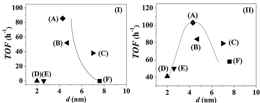
Fig. 7. (I) Benzaldehyde ( T = 413 K, n/F = 1.2 \times 10^{-3} h) and (II) nitrobenzene ( T = 413 K, n/F = 3.7 \times 10^{-3} h) turnover frequency (TOF) as a function of Au particle size ( d ): (A) \blacklozenge Au/γ-Al 2 O 3 ; (B) \blacktriangleleft Au/TiO 2 ; (C) \blacktriangleright Au/ZrO 2 ; (D) \blacktriangle Au/CeO 2 ; (E) \blacktriangledown Au/α-Fe 2 O 3 ; (F) \blacksquare Au/Fe 3 O 4 .
