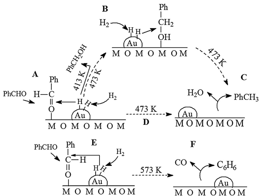
Fig. 10. Proposed reaction mechanism for benzaldehyde hydrogenation over Au/γ-Al 2 O 3 (M = Al) at different reaction temperatures.
