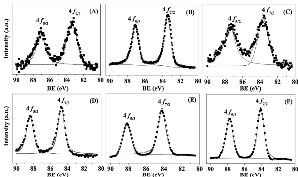
Fig. 5. XPS spectra over the Au 4f region for (A) Au/ \gamma -Al 2 O 3 , (B) Au/TiO 2 , (C) Au/ZrO 2 , (D) Au/CeO 2 , (E) Au/ \alpha -Fe 2 O 3 and (F) Au/Fe 3 O 4 ; experimental data are given by ■ where lines represent data fitting with peak deconvolution.
