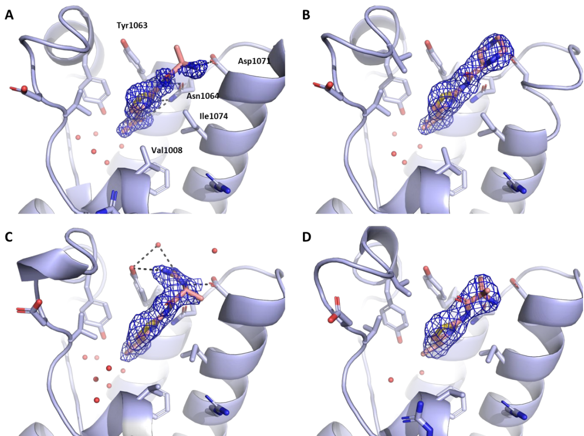
Figure 1. A-D – Crystal structures of the ATAD2 bromodomain in the complex with compounds 1-4. 2Fo-Fc electron density maps are shown in blue. In all figures, conserved water molecules and water molecules involved in bridging polar interactions (dashed lines) between protein and ligand are shown (red spheres).
