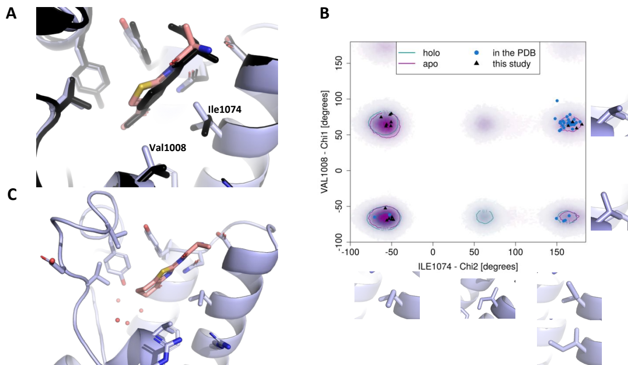
Figure 2. A. Superposition of structures of compounds 1 and 3 (shown in black). B. Populations of different conformers of the residues Val1008 and Ile1074 according to the MD simulations. Individual data points represent the conformational states in crystal structures deposited in the PDB as of 01.03.2019. C. Co-crystal structure of compound 5 bound to ATAD2 bromodomain.
