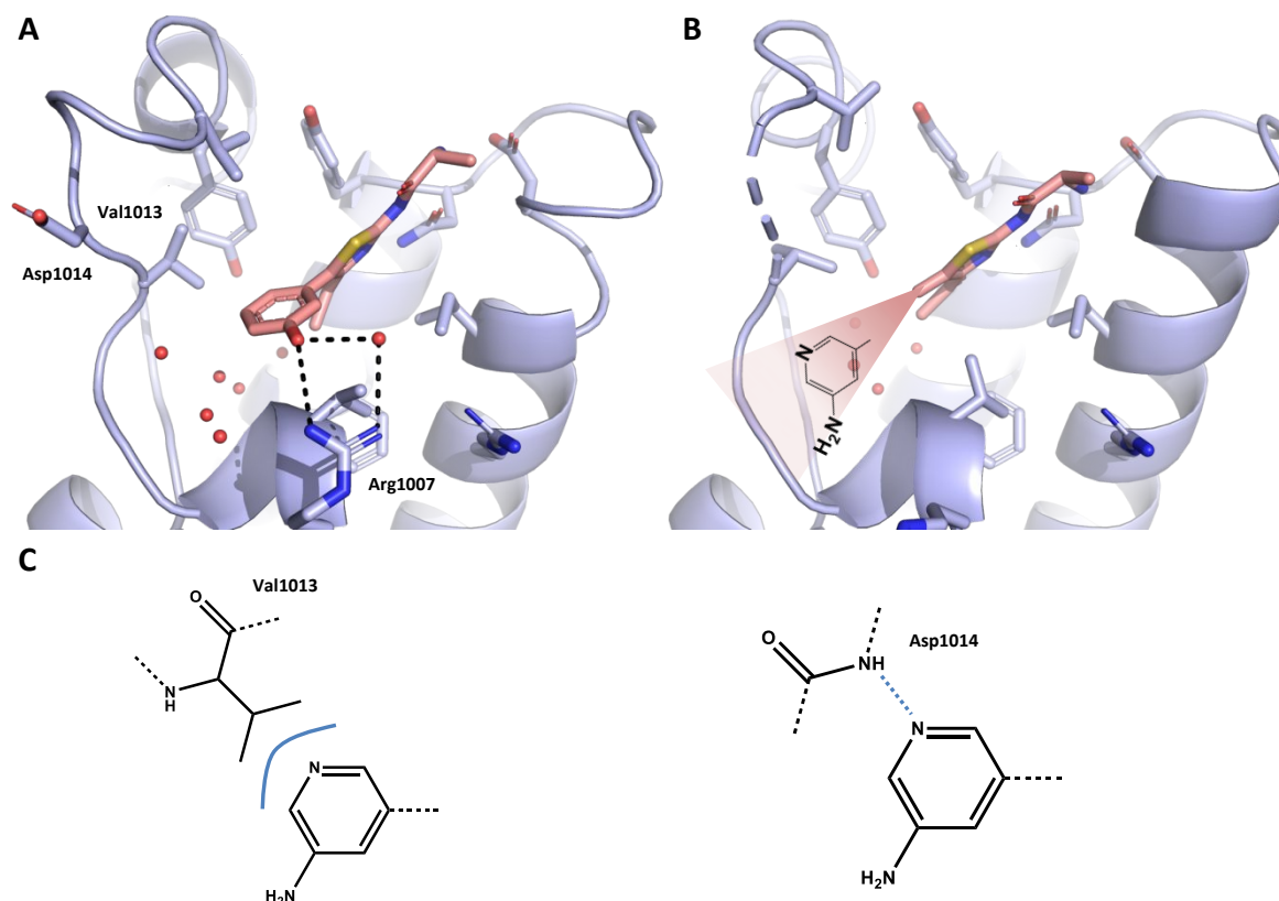
Figure 3. A-B – Crystal structures of the ATAD2 bromodomain in the complex with compounds 6 and 8 , respectively. C – Different binding modes seen in the all-atom MD simulations of compound 8 -ATAD2 bromodomain complex: left – van der Waals interaction between the side chain of Val1013 and amino-pyridine, right – hydrogen bond between the backbone NH of Asp1014 and nitrogen atom of pyridine ring.
