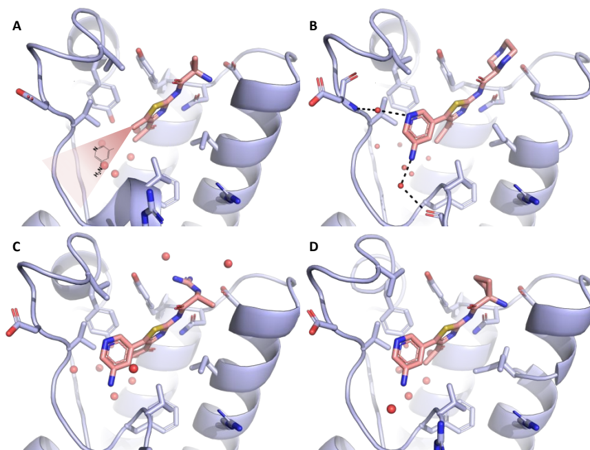
Figure 4. A-D – Crystal structures of the ATAD2 bromodomain in the complex with compounds 11-14 .
