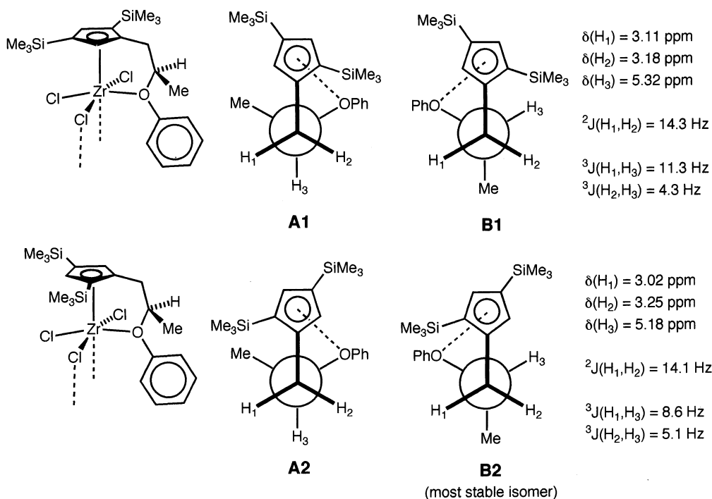
Fig. 4. Conformation analysis on 6d .
