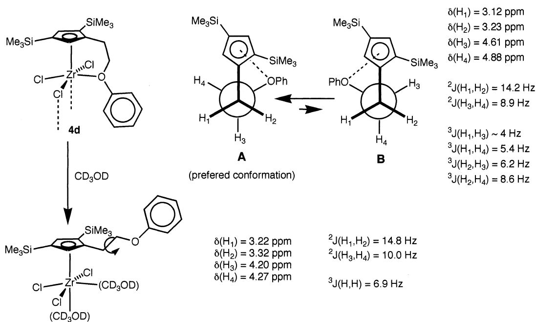
Fig. 2. Conformation analysis on 4d .
