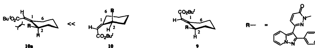
Figure 1. Conformation of cyclohexane ring of 9 and 10 .
