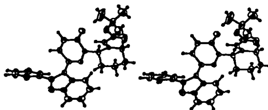
Figure 3. Ortep plot of stereoviews of 9.
