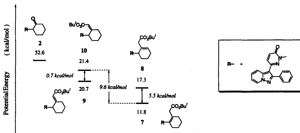
Figure 5. Potential energy diagram of Horner–Emmons products of 2.
