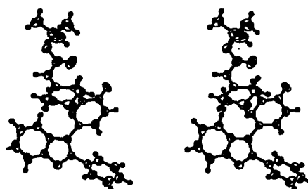
Figure 4. Ortep plot of stereoviews of 10.
