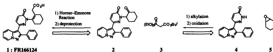
Scheme 1. Synthetic strategy of FR166124 ( 1 ).
