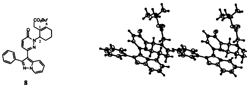
Figure 2. Ortep plot of stereoviews of 8 .
