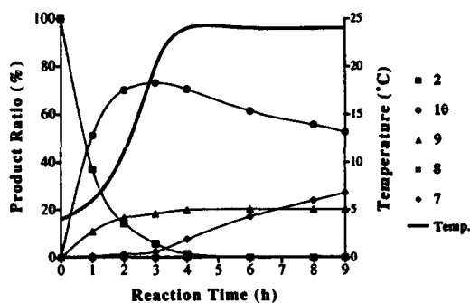
Figure 7 Time-course of Horner–Emmons Reaction at 4 to 24 °C.
