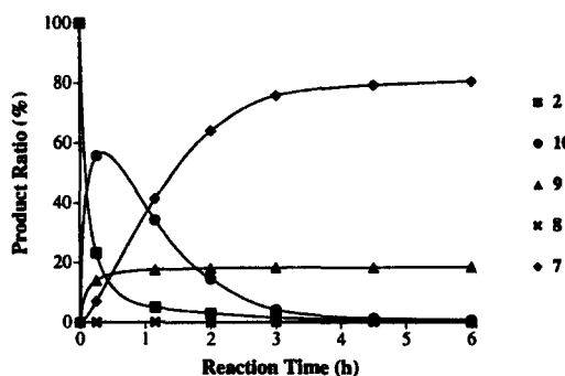
Figure 6 Time-course of Horner–Emmons Reaction at 24 °C.
