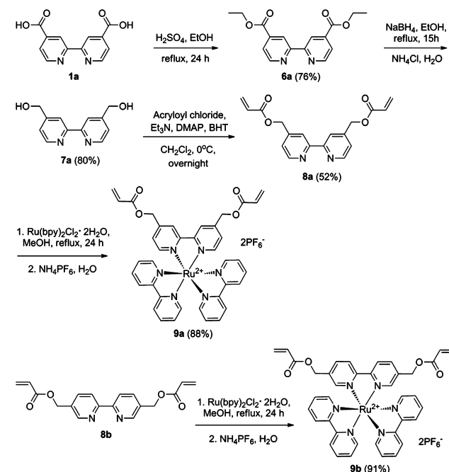
Scheme 3. Synthetic Route to Compounds 9a and 9b
