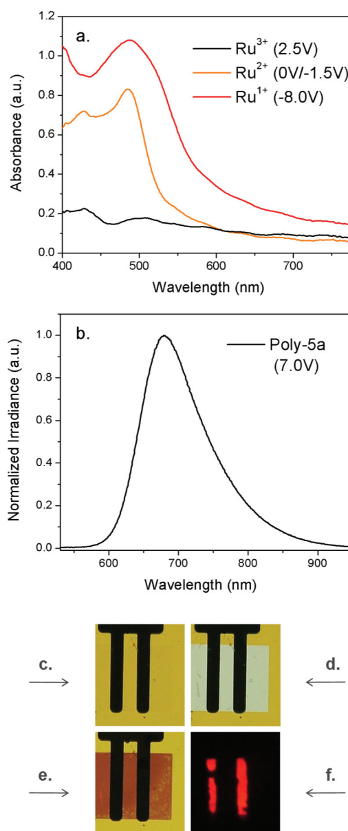
Figure 7. Absorption spectra (a) of a dual EC/EL device pixel as it is operated in the electrochromic mode in the ‘as prepared’ ( \text{Ru}^{2+} ), oxidized ( \text{Ru}^{3+} ), and reduced ( \text{Ru}^{1+} ) states at the indicated voltages along with the corresponding photographs of the pixel in these states: (c), (d), and (e), respectively. Emission spectra (b) of the device pixel operated in the electrochemiluminescent mode at 7 V along with the corresponding photograph (f).
