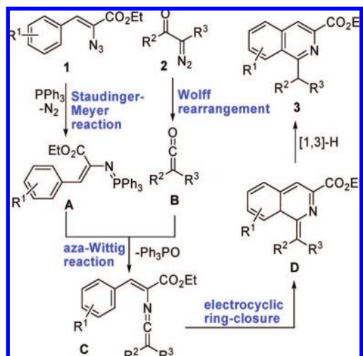
SCHEME 5. Reaction of Asymmetrical 2-Diazo-1,3-diones
