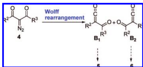
SCHEME 5. Reaction of Asymmetrical 2-Diazo-1,3-diones
