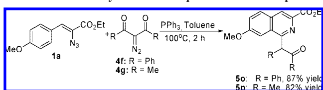
SCHEME 2. The Synthesis of Isoquinolines 5o and 5p
