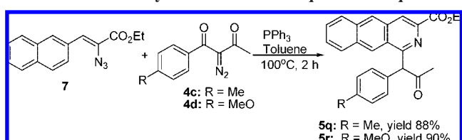
SCHEME 3. The Synthesis of Benzoisoquinolines 5q and 5r
