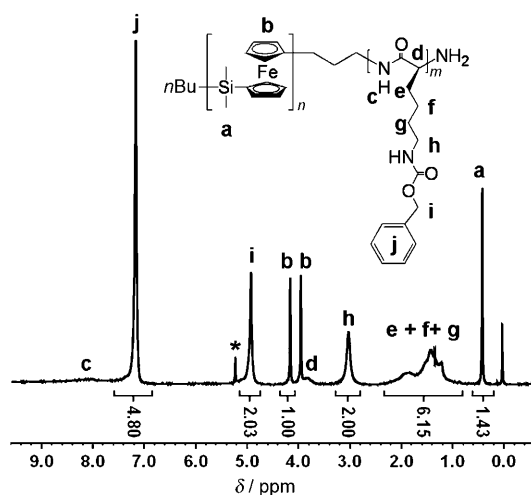
Figure 2. ^1\text{H} NMR spectrum of PFS- b -PZLys 2 in \text{CD}_2\text{Cl}_2 at 25 °C. (* solvent residue)
