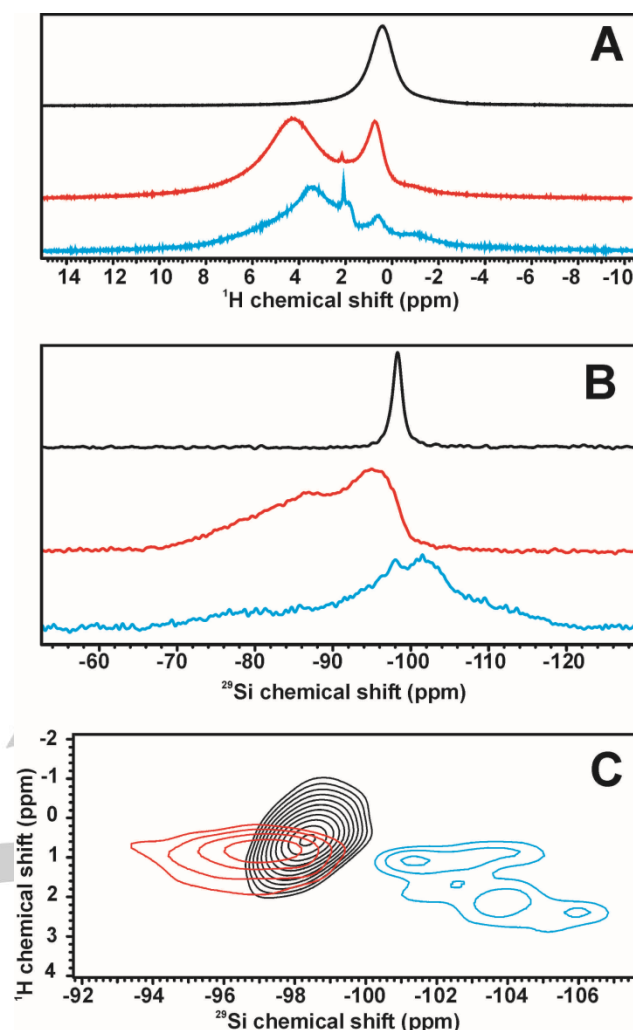
Figure 2. Solid state NMR spectra natural talc (NT), wet-kneaded (WK) and co-precipitated (CP) samples. (A) ^1\text{H} single pulse MAS NMR spectra, (B) ^{29}\text{Si}\{^1\text{H}\} cross-polarization MAS NMR spectra, and (C) ^1\text{H} - ^{29}\text{Si} FSLG HETCOR representation of the results.
