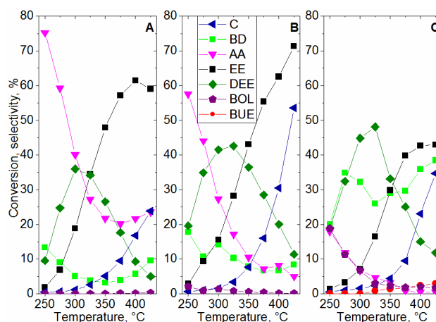
Figure 5. Conversion of ethanol over (A) natural talc, (B) co-precipitated, and (C) wet-kneaded MgO-SiO 2 catalysts as function of reaction temperature. The WHSV was 0.5\text{ g}_{\text{ethanol}}/\text{g}_{\text{cat}}\cdot\text{h}^{-1} at a total gas flow rate of 30\text{ cm}^3\text{ min}^{-1} . The partial pressure of ethanol was about 15 kPa in He. The conversion curve is labelled by letter C. Selectivity curves are given for butadiene (BD), acetaldehyde (AA), ethylene (EE), diethyl ether (DEE), butanol (BOL) and butenes (BUE).
