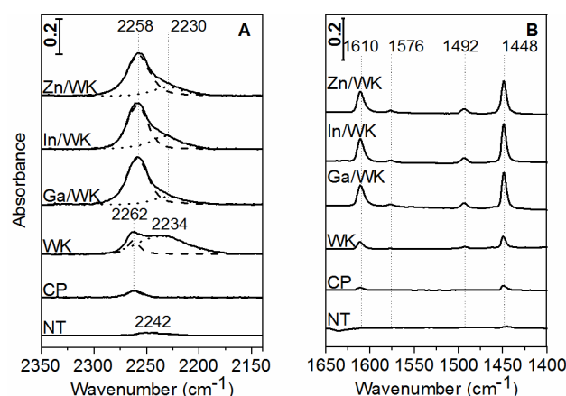
Figure 3. FTIR spectra of adsorbed (A) CDCl 3 and (B) pyridine. The pellets were pre-treated in vacuum at 450 °C for 1 h. The spectra were recorded at room temperature (A) in the presence of CDCl 3 at about 933 Pa pressure, and (B) after adsorption of pyridine at 666 Pa pressure at 200 °C and evacuation at the same temperature for 30 min.
