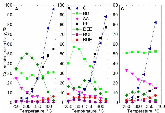
Figure 6. Effect of 1 wt.% (A) \text{Ga}_2\text{O}_3 , (B) \text{In}_2\text{O}_3 , and (C) \text{ZnO} promoter on the conversion of ethanol to butadiene. The WHSV was 0.5 \text{ g}_{\text{ethanol}} \cdot \text{g}_{\text{cat}}^{-1} \text{ h}^{-1} at a total gas flow rate of 30 \text{ cm}^3 \text{ min}^{-1} . The partial pressure of ethanol was about 15 kPa in He. See the Fig.5. for the legends.
