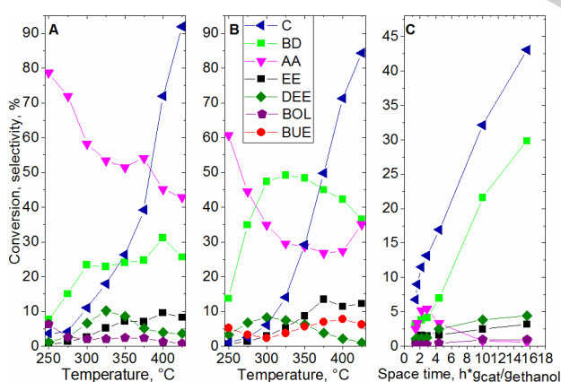
Figure 7. Effect of 1 wt.% \text{ZnO} additive on the activity and selectivity of (A) NT and (B) CP samples in the ETB reaction. The WHSV was 0.5 \text{ g}_{\text{ethanol}} \cdot \text{g}_{\text{cat}}^{-1} \text{ h}^{-1} at a total gas flow rate of 30 \text{ cm}^3 \text{ min}^{-1} . The partial pressure of ethanol was about 15 kPa in He. Section C shows the effect of WHSV on the product yield and conversion over 1 wt.% \text{ZnO}/\text{WK} sample at 300^\circ\text{C} , and ethanol partial pressure of about 15 kPa. The total flow rate was varied in the 5\text{--}120 \text{ cm}^3 \text{ min}^{-1} range. See the Fig.5. for the legends.
