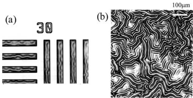
FIGURE 2 Images of rough surface of OCL film. (a) Optical microscope image (Patterned line width is 30 μm); (b) SEM image.
