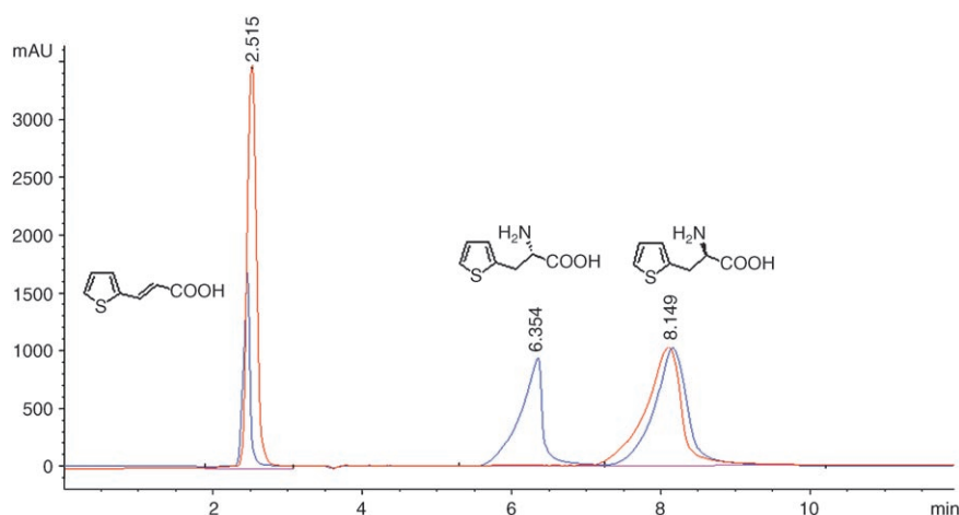
Figure 2. The elution diagram for PAL-catalyzed enantioselective synthesis of D-thiophen-2-yl-alanine. PAL and rac -amino acid, Tris-HCl buffer (pH 8.8); blue trace: after 30 min; red trace: after 2 days.
