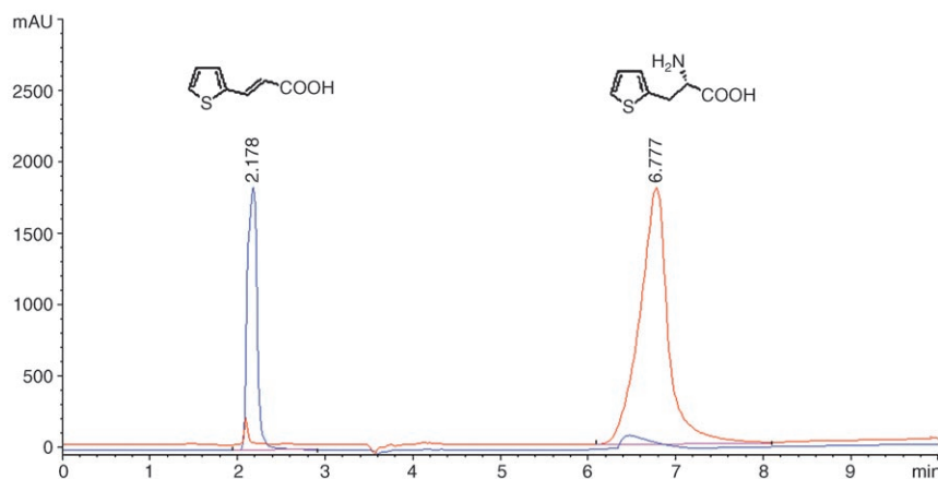
Figure 3. Elution diagram for the synthesis of L-thiophen-2-yl-alanine.
