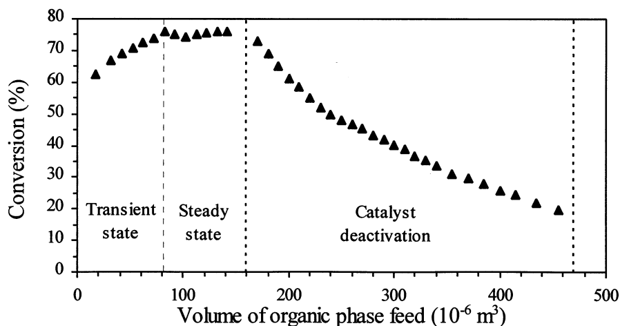
Fig. 6. Typical data obtained with the CPC. Conditions: [dimethylitaconate] = 0.1 \text{ kmol}^{-1} \text{ m}^{-3} , [Rh] = 0.002 \text{ kmol}^{-1} \text{ m}^{-3} , P/\text{Rh} = 3 , total volume = 55 \times 10^{-6} \text{ m}^3 , cyclohexane/water ratio: 1/10; aqueous phase: sodium formate 5 \text{ kmol}^{-1} \text{ m}^{-3} .
