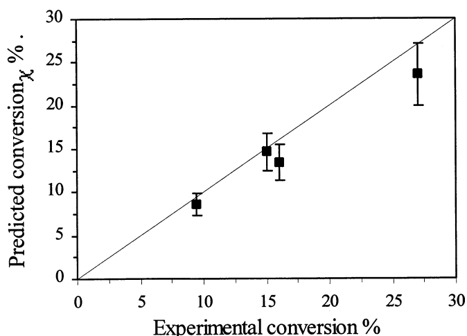
Fig. 7. Comparison between the experimental and the predicted conversion ( \chi_{\text{out}} ). Conditions: T = 300 \text{ K} ; V_R = 52.10 \times 10^{-6} \text{ m}^3 ; = 3.4 \times 10^{-3} \text{ kmol}^{-1} \text{ m}^{-3} ; = 0.117 \text{ kmol m}^{-3} ; Q = 5.3, 9.0, 9.2 and 15.7 \times 10^{-9} \text{ m}^3 \text{ s}^{-1} with \alpha = 0.31, 0.27, 0.37 and 0.27 , respectively.
