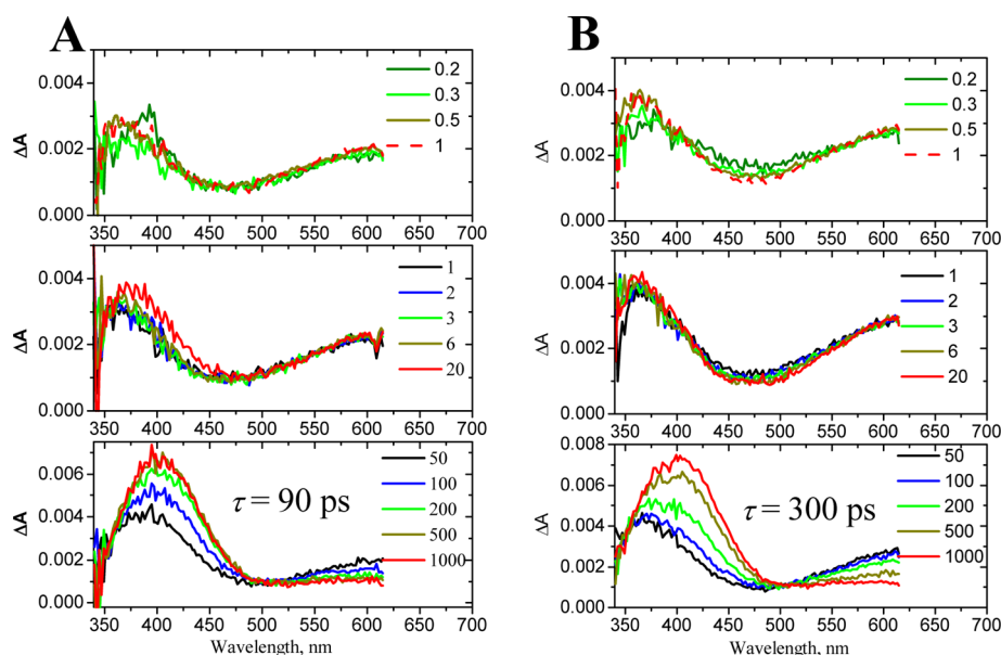
Figure 8. Ultrafast transient absorption spectra of azide 13Bz 3 in MeOH, \tau = 90 ps (singlet nitrene 27s decay at 375 nm and 550–625 nm, and iminoquinone 7Bz 3 formation at 405 nm) (A) and in 2-PrOH, \tau = 300 ps (singlet nitrene 27s decay at 375 nm and 550–625 nm, and iminoquinone 7Bz 3 formation at 405 nm) (B). Time delays between pump and probe pulses are given in picoseconds in the legends.
