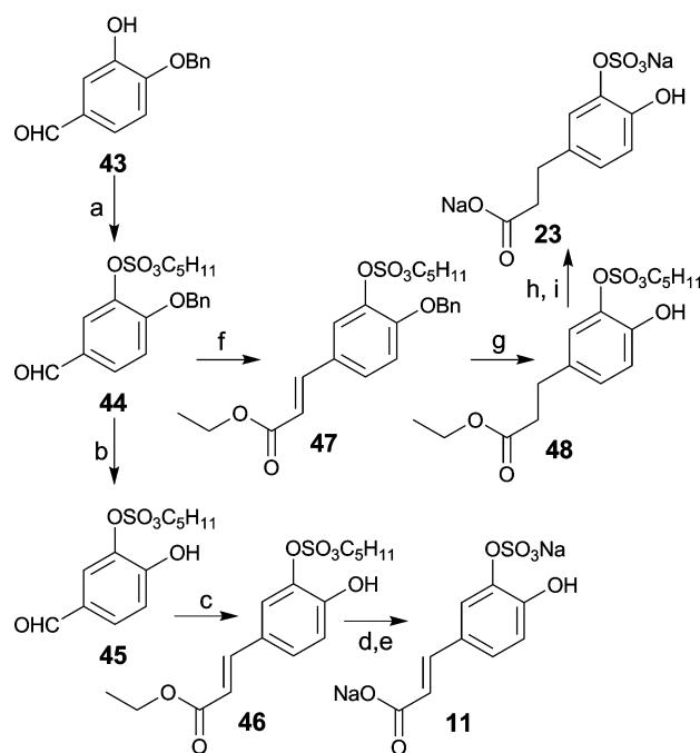
Scheme 3 The preparations of caffeic acid 3'-sulfate 11 , and dihydrocaffeic acid 3'-sulfate 23 . a) \text{Cl-SO}_3\text{-C}_5\text{H}_{11} , DBU, \text{CH}_2\text{Cl}_2 , 91%; b) Cyclohexene, 10% Pd/C, DMF, 94%; c) Ethyl (triphenylphosphoranylidene)acetate, \text{CH}_2\text{Cl}_2 -THF, 83%; d) \text{NaN}_3 , DMF; e) 1 N aq. NaOH then Amberlite® CG-50, d + e: 43%; f) Ethyl (triphenylphosphoranylidene)acetate, \text{CH}_2\text{Cl}_2 -THF, 86%; g) \text{H}_2 , 5% Pd/C, MeOH- \text{H}_2\text{O} , 100%; h) \text{NaN}_3 , DMF; i) 1 N aq. NaOH then Amberlite® CG-50, h + i: 70%.
