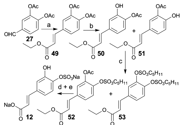
Scheme 4 The preparation of caffeic acid 4'-sulfate 12 . a) Ethyl (triphenylphosphoranylidene)acetate, \text{CH}_2\text{Cl}_2 , 100%; b) Thiophenol, imidazole, NMP, 54% of 50 + 51 ; c) \text{Cl-SO}_3\text{-C}_5\text{H}_{11} , \text{Et}_3\text{N} , DMAP, THF, 80% of 52 ; d) \text{NaN}_3 , DMF; e) 1 N aq. NaOH then Amberlite® CG-50, d + e: 67%.
