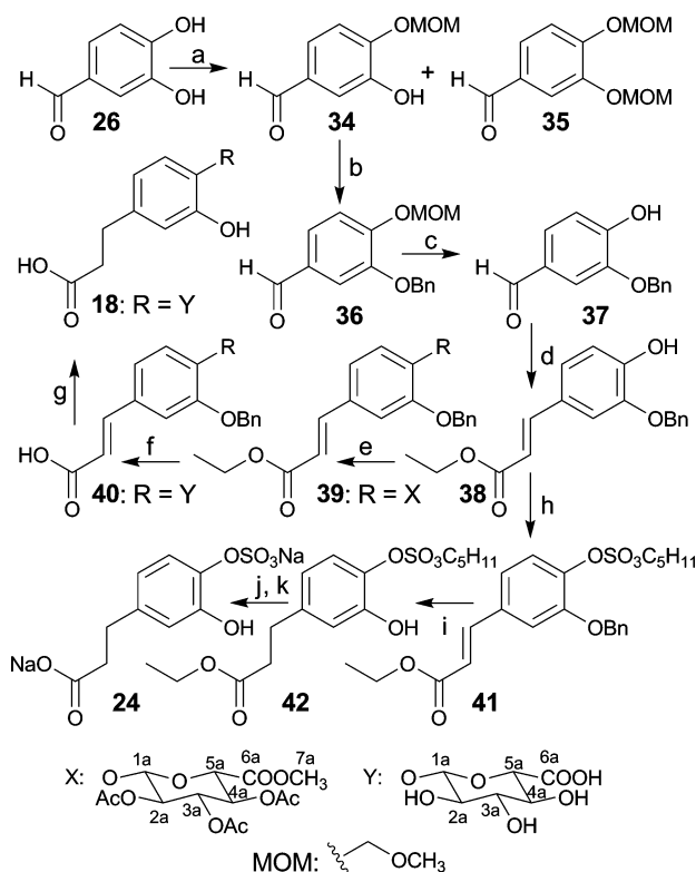
Scheme 2 The preparations of dihydrocaffeic acid 4'- O - \beta -D-glucuronide 18 , and of dihydrocaffeic acid 4'-sulfate 24 . a) Chloromethyl methyl ether, i\text{Pr}_2\text{NEt} , THF; b) Benzyl bromide, \text{K}_2\text{CO}_3 , MeCN; c) 37% HCl, MeOH; a + b + c: 42% d) Ethyl (triphenylphosphoranylidene)acetate, \text{CH}_2\text{Cl}_2 -THF, 56%; e) Compound 25 , \text{BF}_3 etherate, \text{CH}_2\text{Cl}_2 , 73%; f) NaOH, MeOH/ \text{H}_2\text{O} , then Amberlite® IR-120, 78%; g) \text{H}_2 , 5% Pd/C, MeOH- \text{H}_2\text{O} , 100%; h) \text{Cl-SO}_3\text{-C}_5\text{H}_{11} , \text{Et}_3\text{N} , DMAP, THF, 86%; i) \text{H}_2 , 5% Pd/C, MeOH- \text{H}_2\text{O} , 90%; j) \text{NaN}_3 , DMF; k) 1 N aq. NaOH then Amberlite® CG-50, j + k: 34%.
