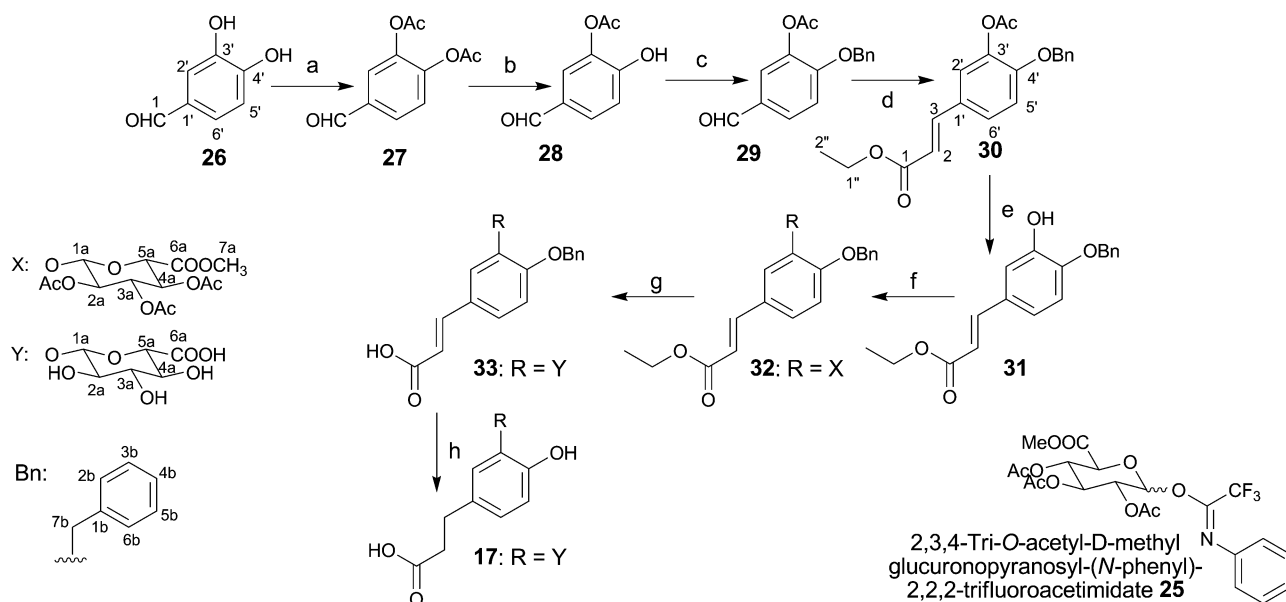
Scheme 1 The preparation of dihydrocaffeic acid 3'- O - \beta -D-glucuronide 17 . a) Acetyl chloride, DBU, CH 2 Cl 2 , 88%; b) Thiophenol, imidazole, NMP, 77%; c) Benzyl alcohol, triphenylphosphine, DEAD, 97%; d) Ethyl (triphenylphosphoranylidene)acetate, CH 2 Cl 2 , 89%; e) NaOMe, dry MeOH–dry CH 2 Cl 2 , 97%; f) 2,3,4-Triacetyl-D-methyl glucuronopyranosyl-( N -phenyl)-2,2,2-trifluoroacetimidate 25 , BF 3 etherate, CH 2 Cl 2 , 76%; g) NaOH, MeOH–H 2 O, then Amberlite® IR-120, 73%; h) H 2 , 5% Pd/C, MeOH–H 2 O, 96%.
