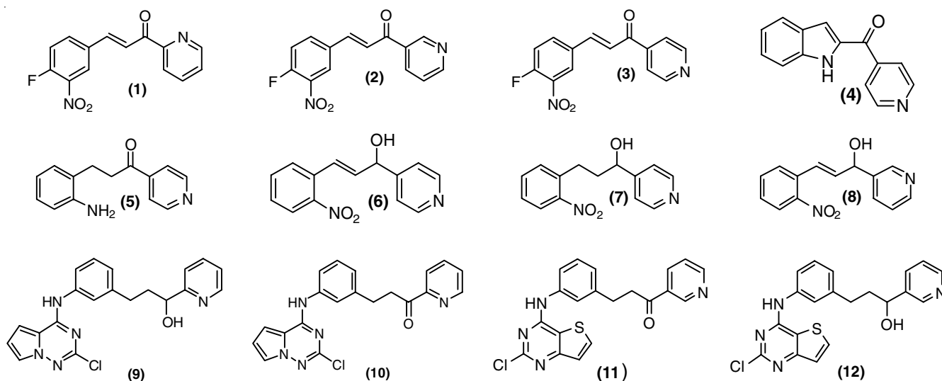
Structure of synthesized compounds 1-12
