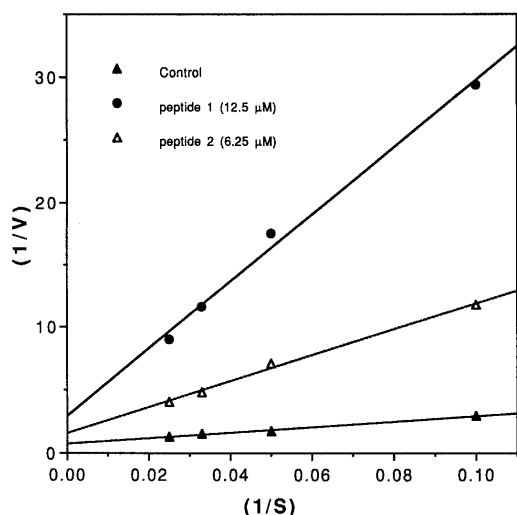
Fig. 5. Lineweaver-Burk Plot of Papain Activity
