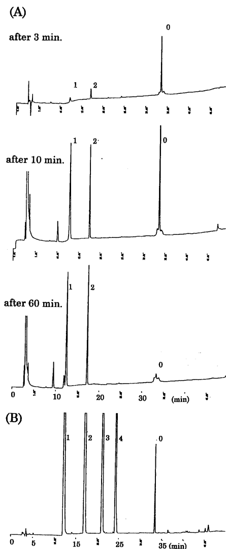
Fig. 6. HPLC Analyses of Suc-Ala-Val-Val-Ala-Ala-pNA Digestion by Papain
