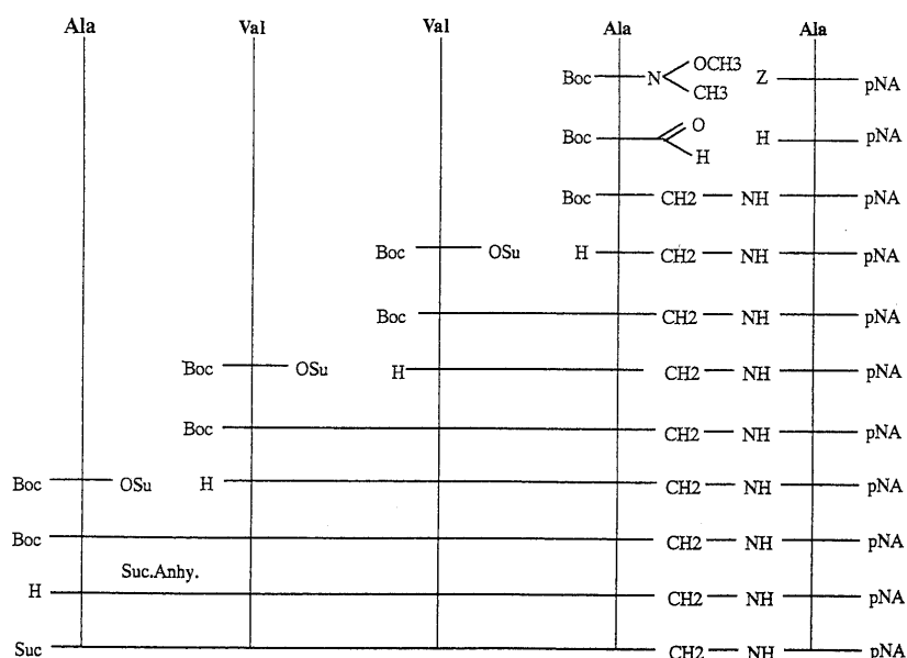
Fig. 2. Synthetic Scheme for the Pseudo-Peptide Analogs
