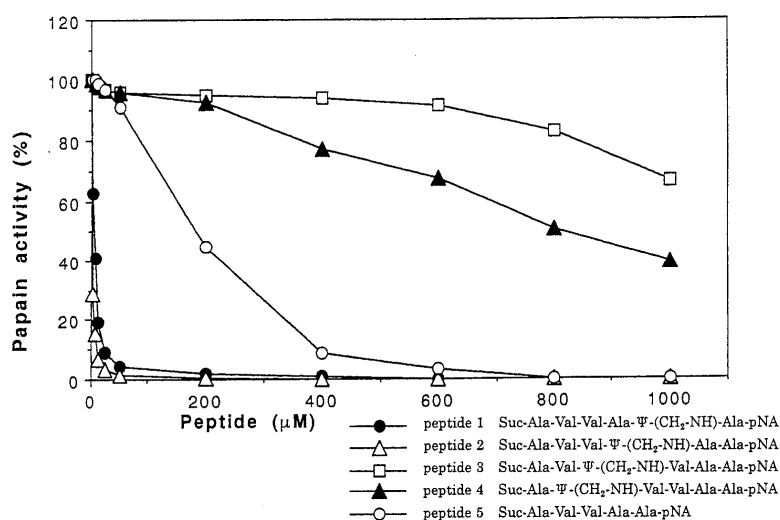
Fig. 3. Inhibition of Papain Activity by Suc-Ala-Val-Val-Ala-Ala-pNA Analogs
