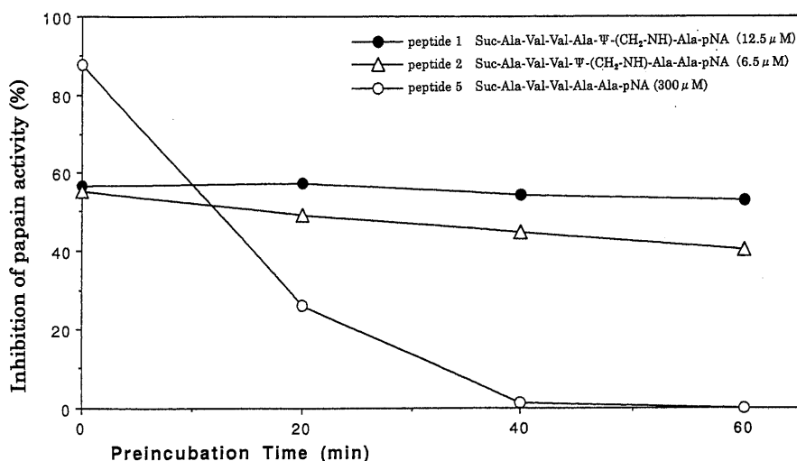
Fig. 4. Inactivation of the Papain-Inhibitory Activity of Suc-Ala-Val-Val-Ala-Ala-pNA analogs Preincubated with Papain
