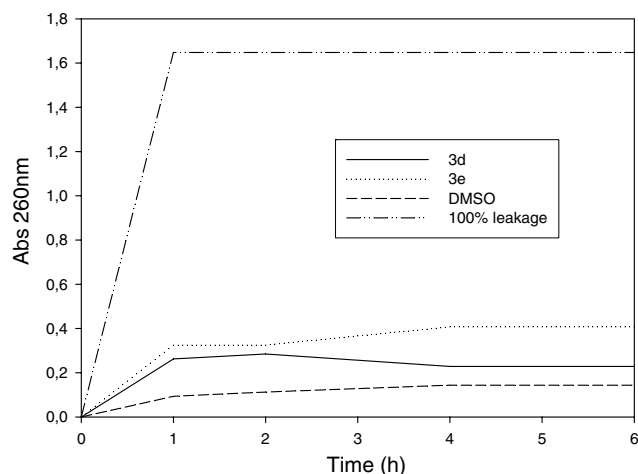
Figure 4. Release of 260-UV absorbing materials from cells of S. cerevisiae incubated with 10 \times CFM of compounds 3d and 3e for 2, 4, and 6 h.
