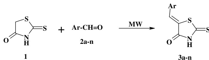
Scheme 1. General methodology for the preparation of arylidenerhodanines 3a–3n . Ar = a: \text{C}_6\text{H}_5 ; b: 4\text{-ClC}_6\text{H}_4 ; c: 4\text{-BrC}_6\text{H}_4 ; d: 4\text{-FC}_6\text{H}_4 ; e: 4\text{-CF}_3\text{C}_6\text{H}_4 ; f: 2\text{-FC}_6\text{H}_4 ; g: 2\text{-CF}_3\text{C}_6\text{H}_4 ; h: 4\text{-CH}_3\text{C}_6\text{H}_4 ; i: 4\text{-CH}_3\text{OC}_6\text{H}_4 ; j: 3,4\text{-OCH}_2\text{OC}_6\text{H}_3 ; k: 3,4,5\text{-tri-CH}_3\text{OC}_6\text{H}_2 ; l: 2-pyridyl; m: 3-pyridyl; n: 4-pyridyl.
