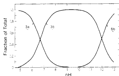
Figure 2. Fractional amount of each species of eq 3 as a function of pH for K_{eq} = 10^{-6} , pK_a^{SH} = 6 , pK_a^{Im} = 6.69 . The pH dependence of the fraction of 6a is a bell-shaped curve with the maximum value of 9.96 \times 10^{-7} at pH 9.3.
