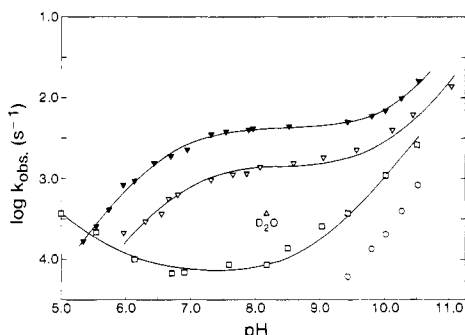
Figure 1. Plot of observed pseudo-first-order rate constants vs. pH at 37.6 \pm 0.3 °C; 3 in ethanolic buffer (▼); 3 in aqueous buffer (▽); 4 in ethanolic buffer, □; 5 in ethanolic buffer (○). (Δ) represents the hydrolysis of 3 in D 2 O solution at pD(H) = 8.2. (For actual conditions, see Experimental Section.)
