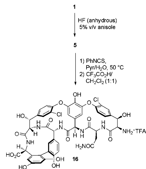
Figure 4. Target molecules.
