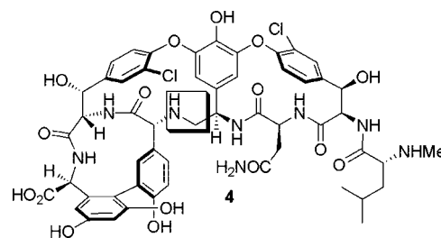
Figure 2. [ \Psi [CH 2 NH]Tpg 4 ]Vancomycin aglycon.
