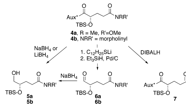
SCHEME 2. Chemoselective Transformations
