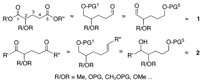
SCHEME 1. Representative Series of C1–C5 Fragments Available from 3 and Michael Acceptors
