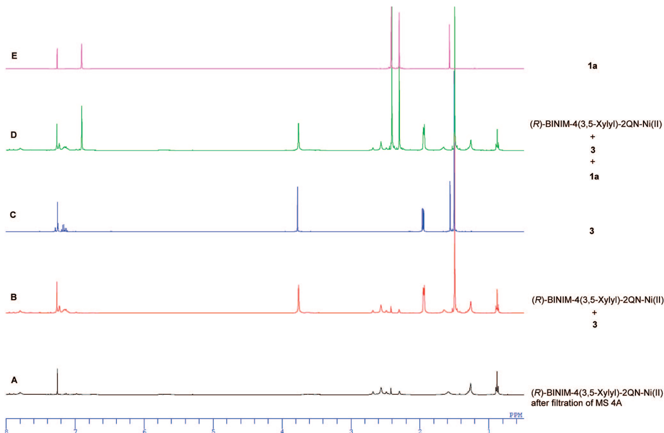
FIGURE 2. ^1\text{H} NMR study of ( R )-BINIM-4(3,5-xylyl)-2QN complex in \text{CDCl}_3 (see Supporting Information for good resolution).
