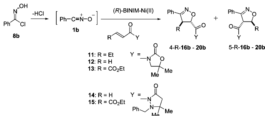
SCHEME 3. Reactions Between Benzonitrile Oxide ( 1b ) and Olefins 11–15 Catalyzed by ( R )-BINIM-Ni(II)
