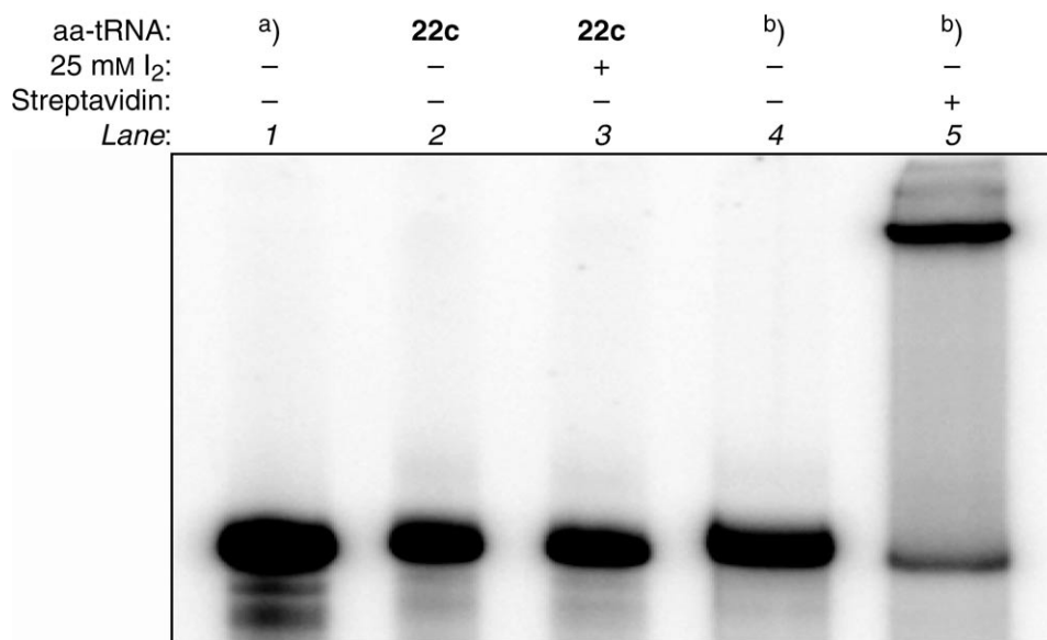
Fig. 1. Autoradiogram of the streptavidin-gel-shift analysis of ligation products [3'(2')\text{-O-}\{N\text{-}[(\text{biotinylamino})\text{caproyl}]\text{-L-methionyl-pCpA and } [5'\text{-}^{32}\text{P}]\text{-tRNA}(-\text{CA})^{\text{Phe}}] . The samples were run on 7.5M urea/10% polyacrylamide gel with 1\times\text{TBE} buffer at 30 W (TBE = Tris/boric acid/ \text{Na}_2\text{edta} ). a) aa-tRNA = Escherichia coli tRNA( -\text{CA} ) Phe . b) aa-tRNA = \{N\text{-}[(\text{biotinylamino})\text{caproyl}]\text{-L-methionyl}\} -tRNA.
