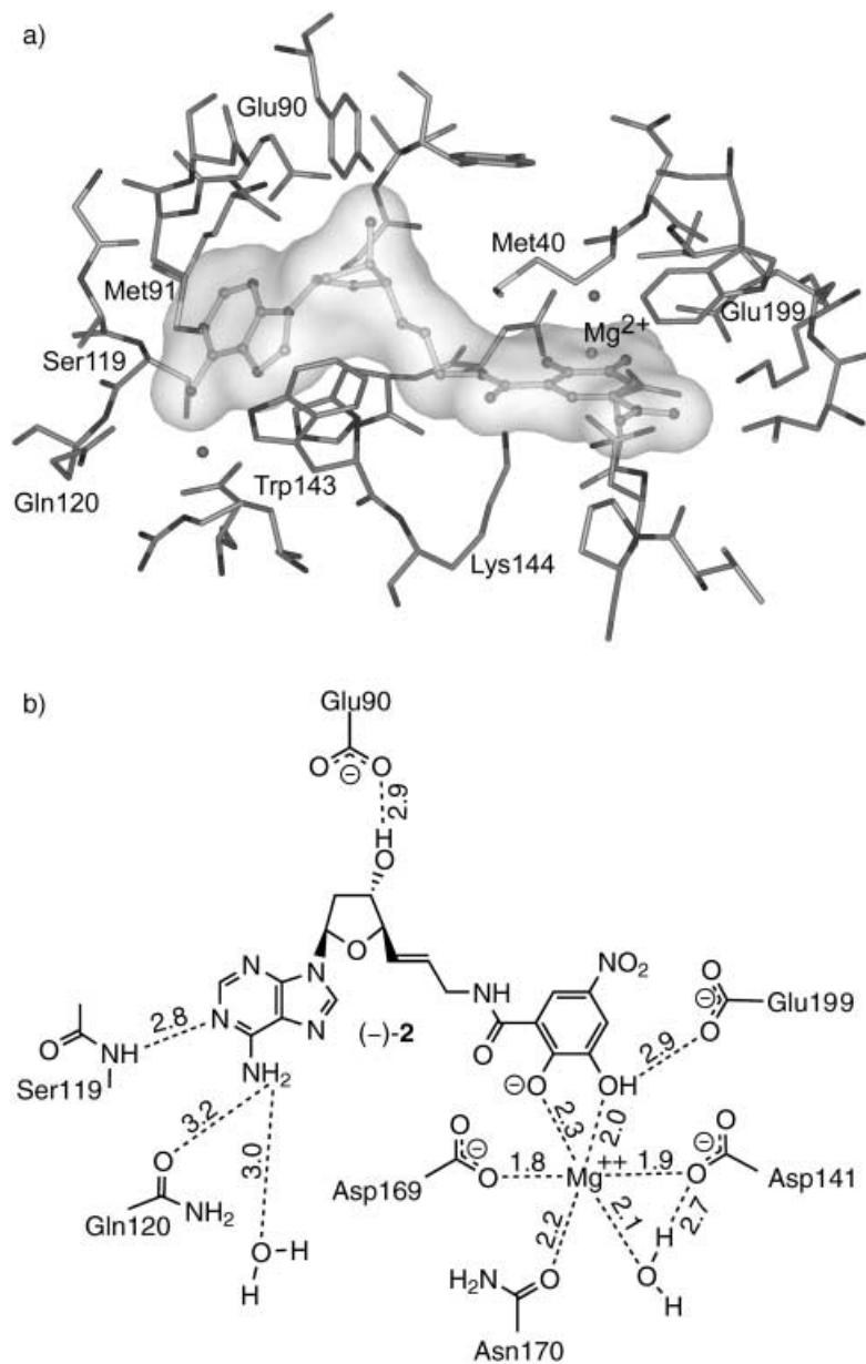
Fig. 1. a) Computer-modeled ternary complex between COMT, Mg^{2+} , and bisubstrate inhibitor (-)-2 . The Connolly surface of the inhibitor is shown. b) Schematic drawing of the H-bonding and metal-ion interactions (dashed lines) in the ternary complex. Distances are given in Å.
