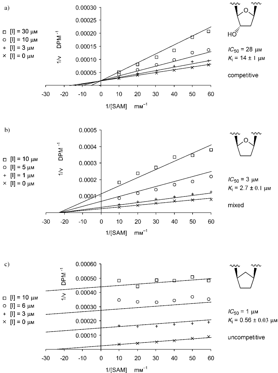
Fig. 3. Lineweaver–Burk plots of reciprocal enzymatic activity vs. reciprocal SAM concentration for varying concentrations of inhibitors (–)- 2 (a), (–)- 3 (b), and (+)- 4 (c) at saturating benzene-1,2-diol concentration. DPM = decays per min.
