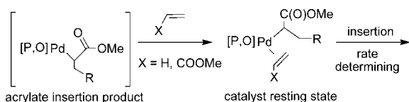
Scheme 1. Rate Limiting Step of Copolymerization
