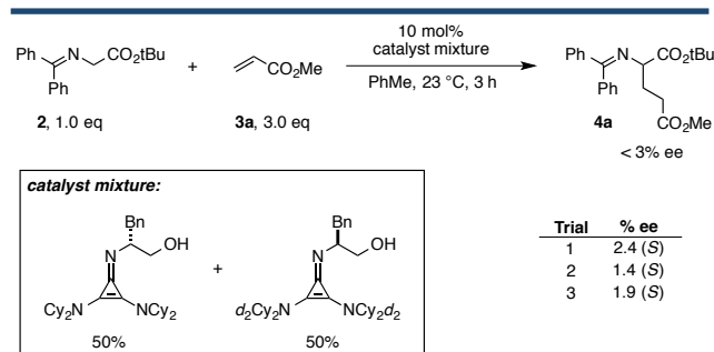
Figure 7. Labeling studies as an experimental probe of CH...O interaction.
