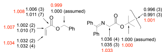
43 44 45 46 47 48 49 50 51 52 Figure 6. Comparison of experimental (black) and predicted (red) ^{13}\text{C} KIEs
