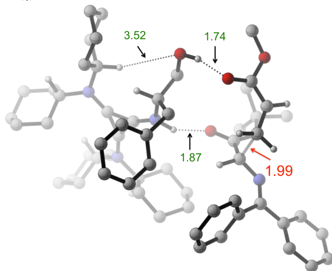
Figure 4. Transition structures leading to major ( S ) enantiomer of product 4a that utilize mono-coordinated binding modes 5a and 5b . Most hydrogen atoms have been removed for clarity. All transition structures are oriented with the acrylate in the foreground and the enolate in the background.
