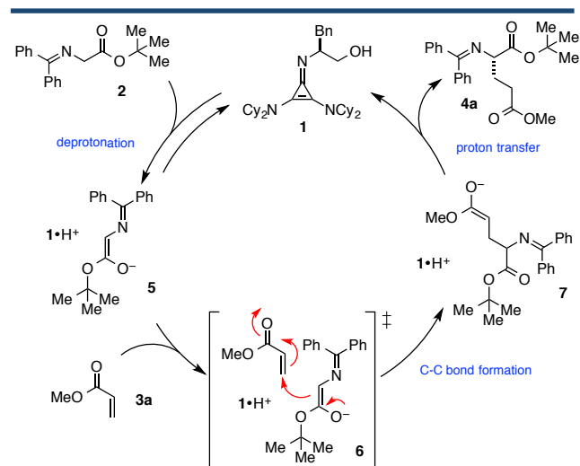
Scheme 2. Proposed mechanism based on experimental KIEs.
