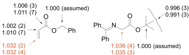
Figure 1. Experimental 13 C KIEs for reaction of 2 and 3b catalyzed by 1 . The two sets of KIEs for each carbon represent two independent experiments and the numbers in parentheses represent the standard deviation in the last digit as determined from six measurements. KIEs for the bond-forming carbon atoms are shown in red.
