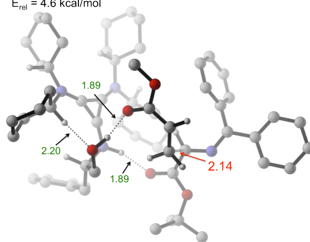
21 22 23 24 25 26 27 28 29 30 31 32 33 34 35 36 37 38 39 40 41 42 Figure 5. Transition structures leading to minor ( R ) enantiomer of product 4a that utilize mono-coordinated binding modes 5a and 5b . Most hydrogen atoms have been removed for clarity. All transition structures are oriented with the acrylate in the foreground and the enolate in the background.
