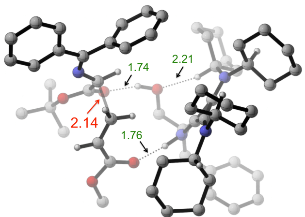
Figure 4. Transition structures leading to major ( S ) enantiomer of product 4a that utilize mono-coordinated binding modes 5a and 5b . Most hydrogen atoms have been removed for clarity. All transition structures are oriented with the acrylate in the foreground and the enolate in the background.
