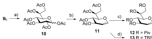
Scheme 3. Reagents and conditions: a) H 2 SO 4 , Ac 2 O, CHCl 3 , 0 °C → RT, 82 %; b) HBr, AcOH, Ac 2 O, CH 2 Cl 2 , RT; Zn, CuSO 4 , AcONa, AcOH, H 2 O, RT, 91 % for 2 steps; c) Na, MeOH, RT; PivCl, DMAP, Py, RT, 82 % for 2 steps; d) Na, MeOH, RT; TBDMSCl, Im, DMF, 0 °C → RT, 95 % for 2 steps.
