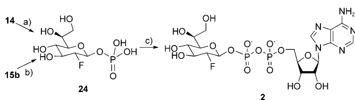
Scheme 6. Reagents and conditions: a) \text{H}_2 , Pd/C; TBAOH, \text{H}_2\text{O} , RT, quant; b) \text{H}_2 , Pd/C; TBAF, THF, 55% for 2 steps; c) AMP-morpholidate, 1H-tetrazole, Py, RT (56%).
