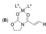
FIGURE 3. N -Enoyl oxazolidinones and their 1,5-metal binding complexes as useful dienophiles for Diels–Alder reactions developed by the Evans group. Active complex A formed from chiral oxazolidinone and achiral ML_2 catalyst; active complex B formed from achiral oxazolidinone and chiral ML_2^* catalyst.
