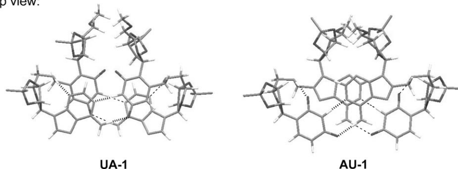
Fig. 1. Front and top view of the Amber*-calculated duplexes UA-1 and AU-1
