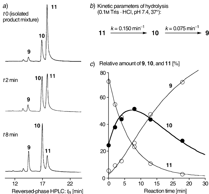
Fig. 3. a) Reversed-phase HPLC traces (detection at 260 nm) obtained by incubating an isolated aminoacylation product mixture in 0.1M aqueous Tris·HCl (pH 7.4) at 37°. b) Independently determined kinetic parameters of hydrolysis for the diacylated product 11 and the monoacylated product 10 . c) Measured (points) and calculated (lines) composition of a hydrolysis reaction mixture obtained according to a) at pH 7.4 and 37° (for details see Exper. Part ).
