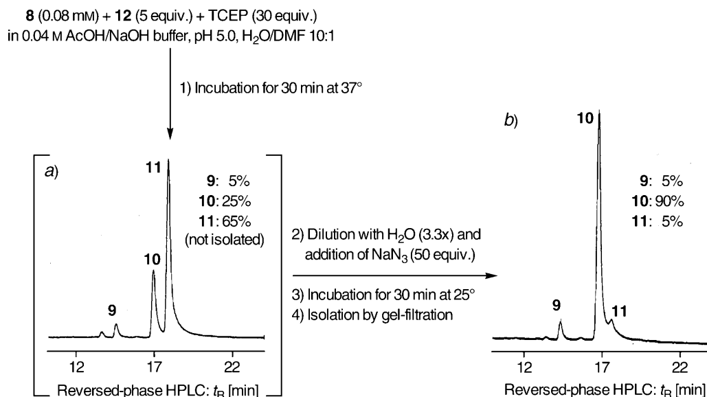
Fig. 4. Conditions for the preparation and isolation of the monoacylated RNA sequence 10 and reversed-phase HPLC traces (detection at 260 nm) of a) the intermediate and b) the final product mixture
