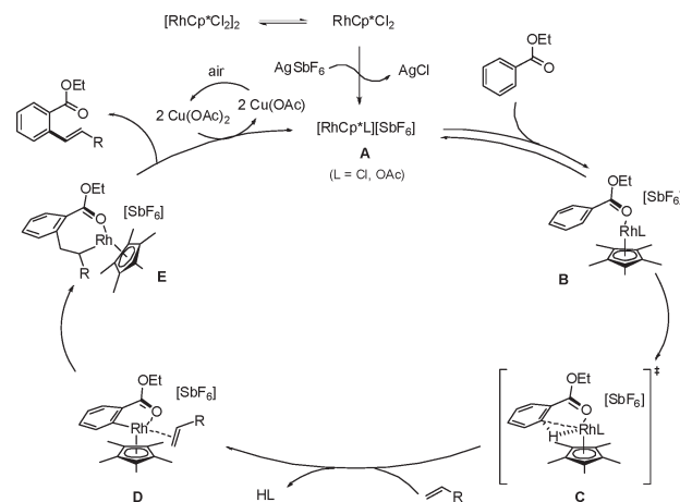
Scheme 4. Proposed Mechanism of Ester-Directed Olefination
