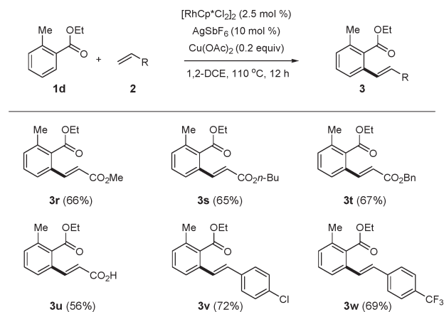
Scheme 3. Ortho -olefination of Ethyl Benzoates a
