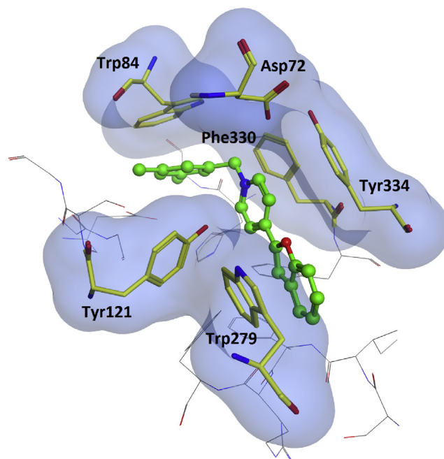
Fig. 2. Illustrative interaction of compound 5e with AChE active site. The key residues are showed by yellow color. (For interpretation of the references to colour in this figure legend, the reader is referred to the web version of this article.)
