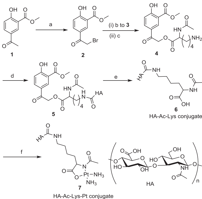
Scheme 2. Synthesis of HA-Ac-Lys-Pt conjugate; Reagents and conditions: a) \text{CuBr}_2 , \text{CHCl}_3/\text{EtOAc} , 40–50 °C, 3–4 h, 85%; b) \text{Ac-Lys(Boc)-OH} , \text{K}_2\text{CO}_3 , \text{MeCN} , overnight; c) \text{TFA}/\text{DCM} , 2–3 h, 85%; d) HA, DMTMM, \text{H}_2\text{O} , 37 °C, 48 h, pH ~4–5, 20 mg/mL; e) h\nu , photolysis, \text{H}_2\text{O} , 2–4 h; f) \text{Pt}[\text{H}_2\text{O}]_2[\text{NH}_3]_2 , \text{H}_2\text{O} , pH ~5, 50 °C, 48 h.
