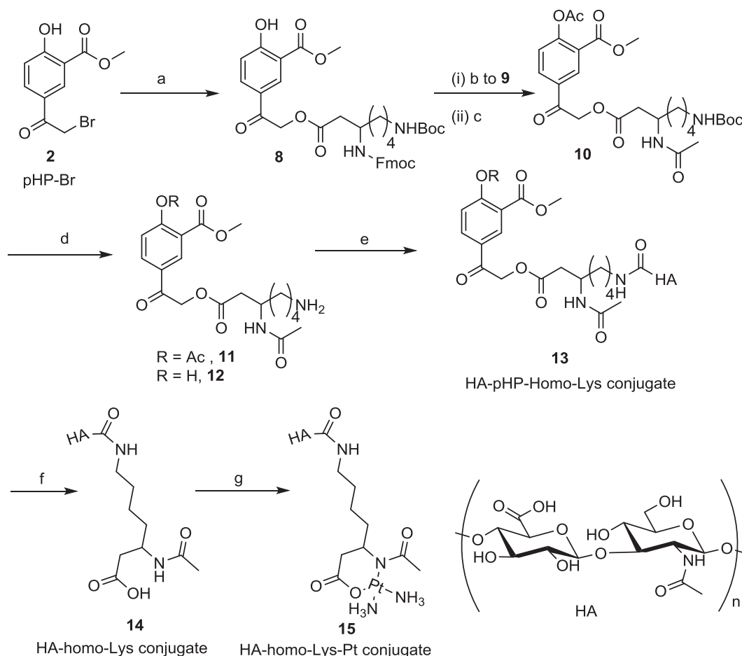
Scheme 3. Synthesis of HA-Ac-homo-Lys-Pt conjugate; Reagents and conditions: a) Fmoc-homo-Lys(Boc)-OH, K_2CO_3 , MeCN, overnight, 86%; b) Piperidine, DMF, 0 °C, 30 min; c) CH_3COCl , CH_2Cl_2 , Et_3N , 0 °C, 30 min, 92%; d) TFA/DCM, 2–3 h, 11 –80%; e) HA, DMETMM, H_2O , 37 °C, 48 h, pH ~4–5, 20 mg/mL; f) hv, photolysis, H_2O , 2–4 h, 100%; g) Pt[H_2O]_2[NH_3]_2 , H_2O , pH ~5, 50 °C, 48 h.
