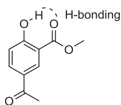
Fig. 2. Intramolecular H-bonding of methyl 5-acetylsalicylate.
